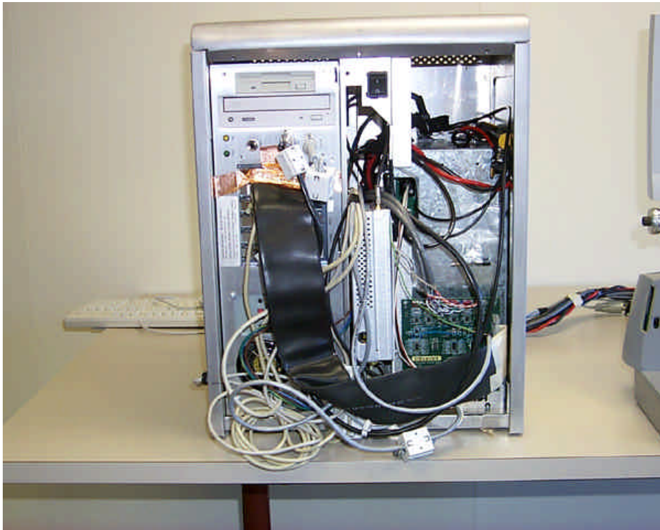
Workstation Electronic Enclosure (WEE) - Cover Off
