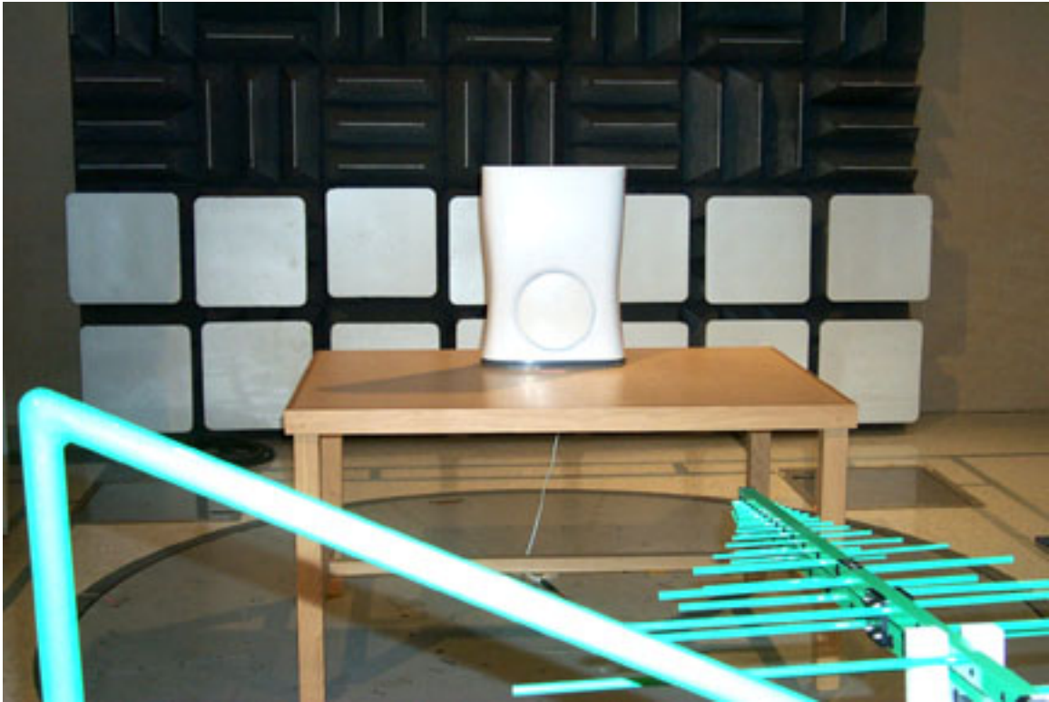
Radiated Emissions Test Setup (Ionizer)
