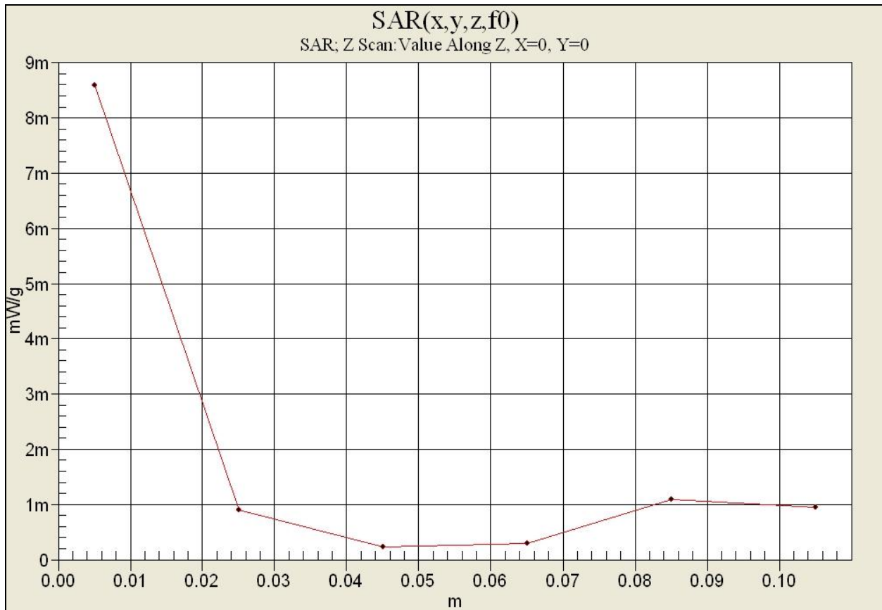
Plot 2. 2401.92MHz Right Head (Z Scan)
