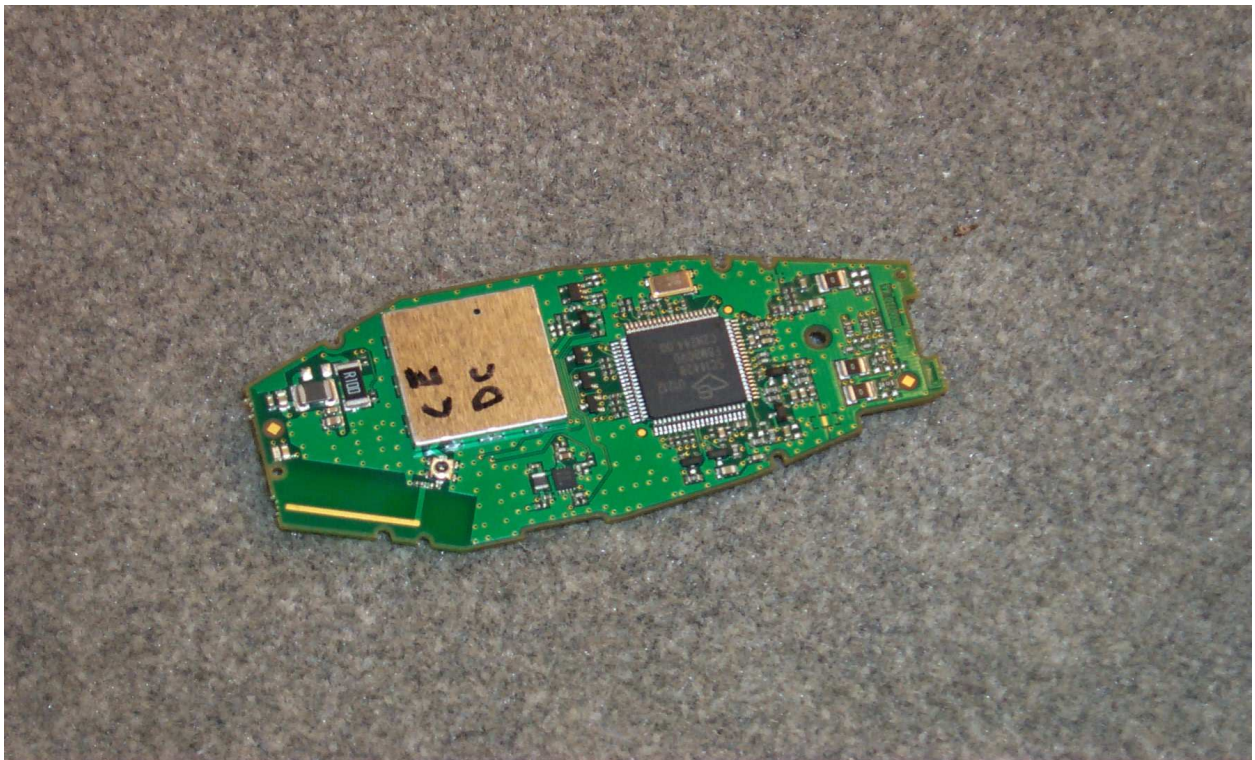
XT-1H PCB Bottom
