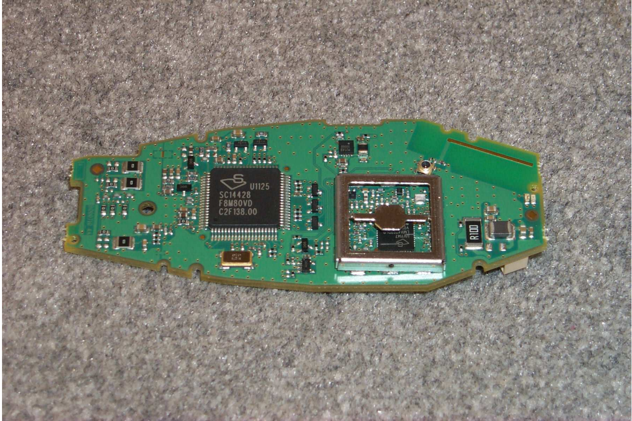
RF Shield Removed from PA Section
