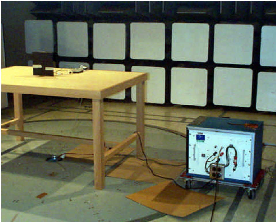
Conducted Emissions
