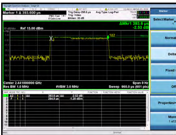
8-DPSK 3DH1
