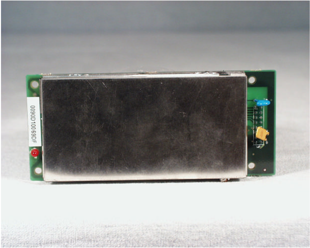
Front view of the complete RF transceiver (RF cans installed)
