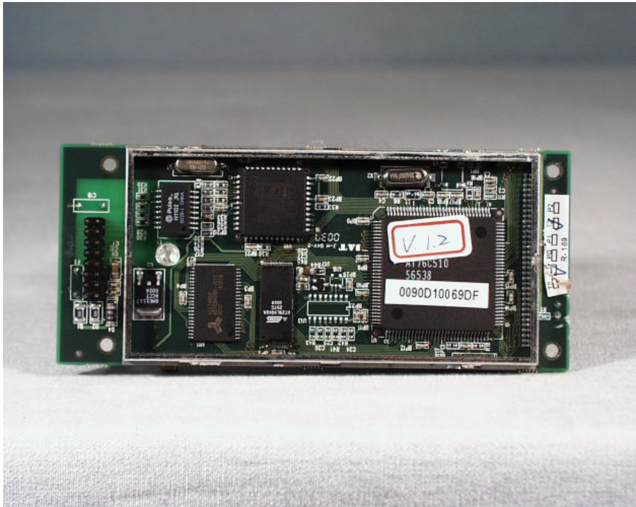
Back view of the complete RF transceiver (RF cans removed)
