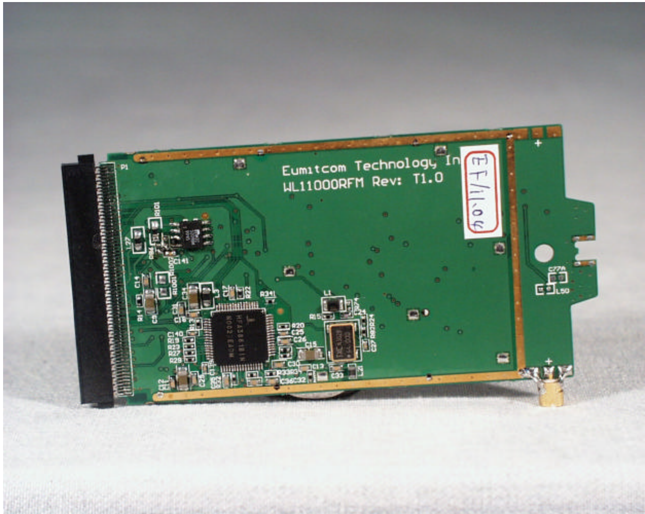
Back view of the Eumitcom PCMPIA RF transceiver
