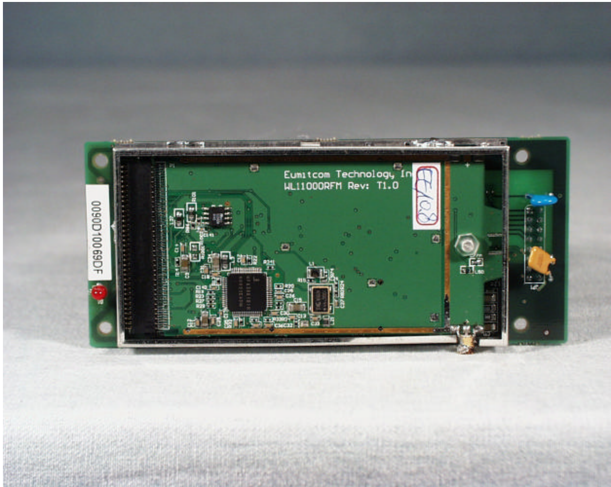
Front view of the complete RF transceiver (RF cans removed)
