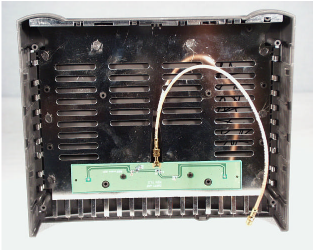
Antenna board
