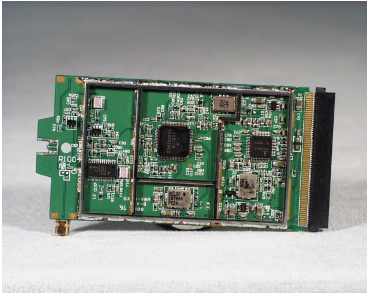
Front view of the Eumitcom PCMPIA RF transceiver (RF cans removed)
