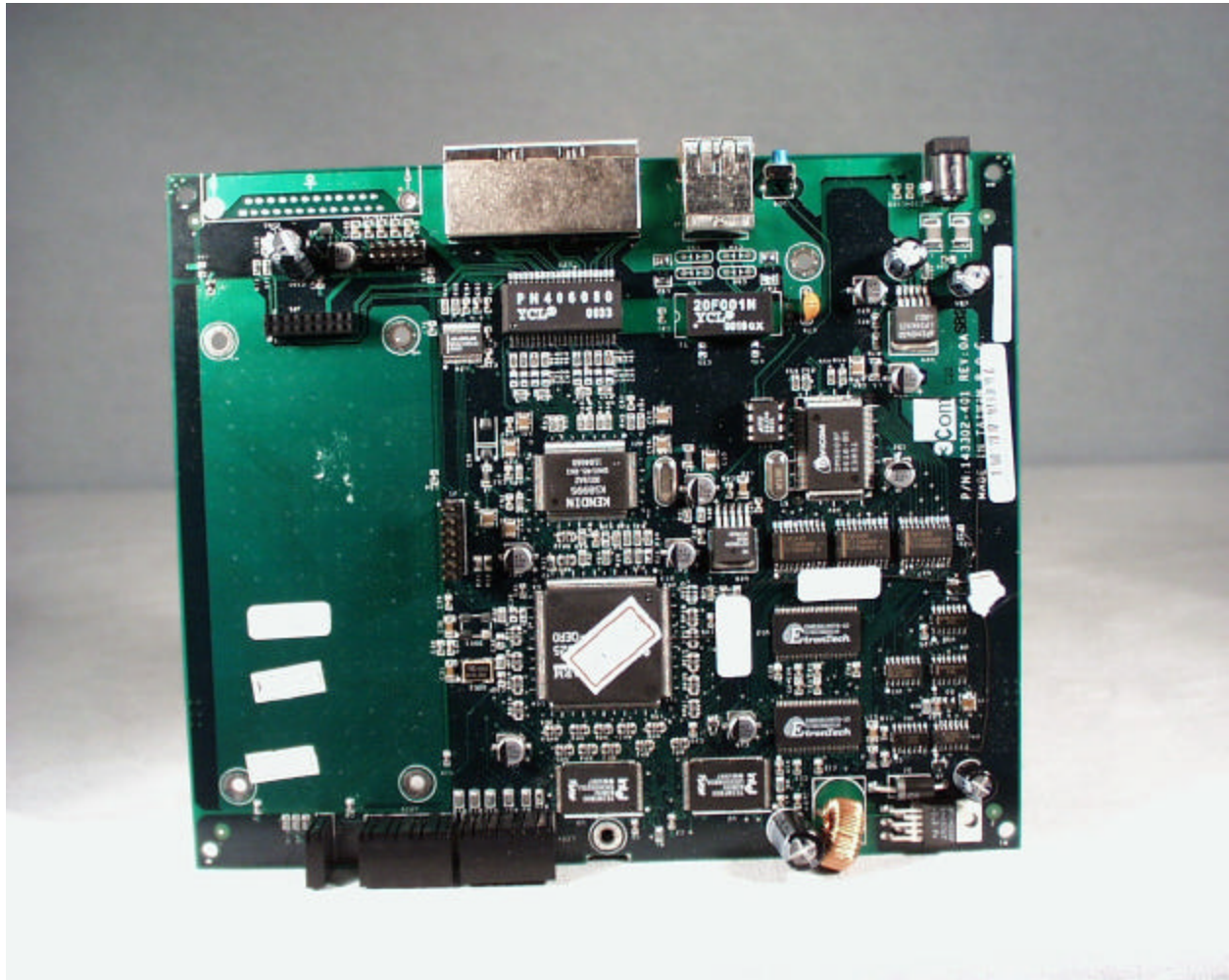
Front view of the digital board
