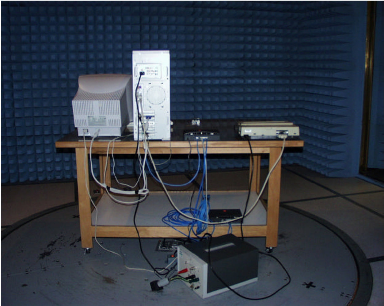
Back view worst case radiated emissions
