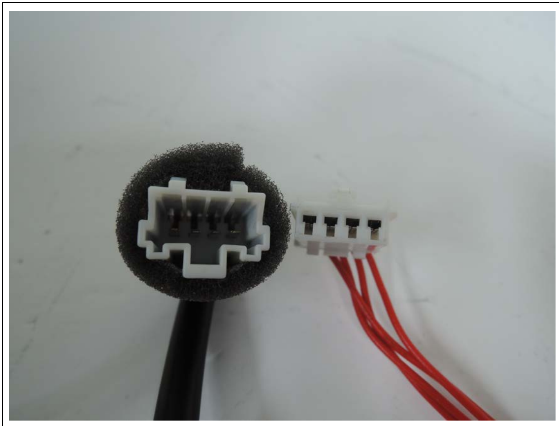
<Antenna Connector Type>
