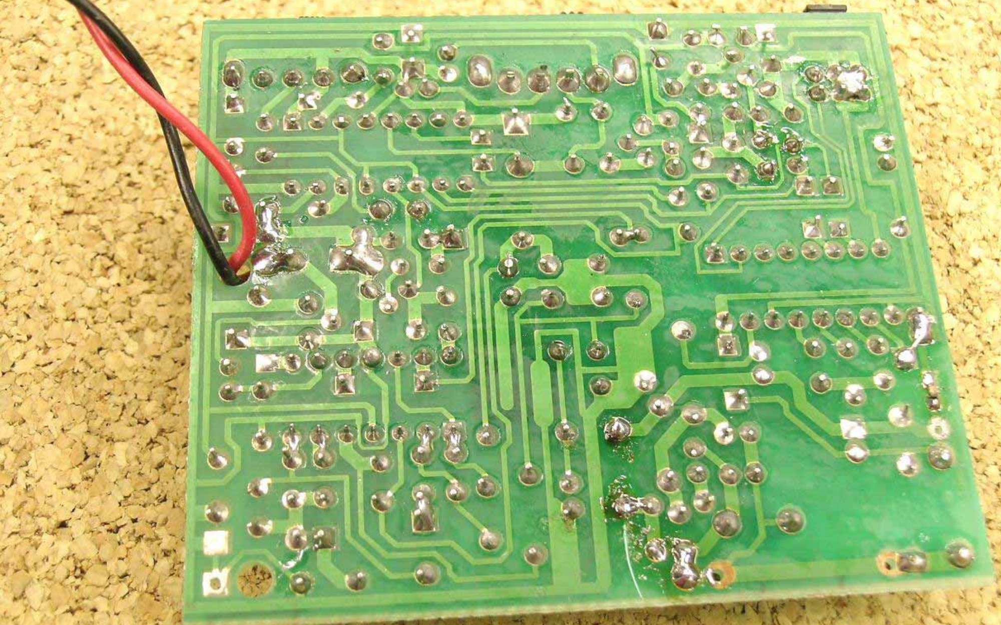
PCB (bottom)
