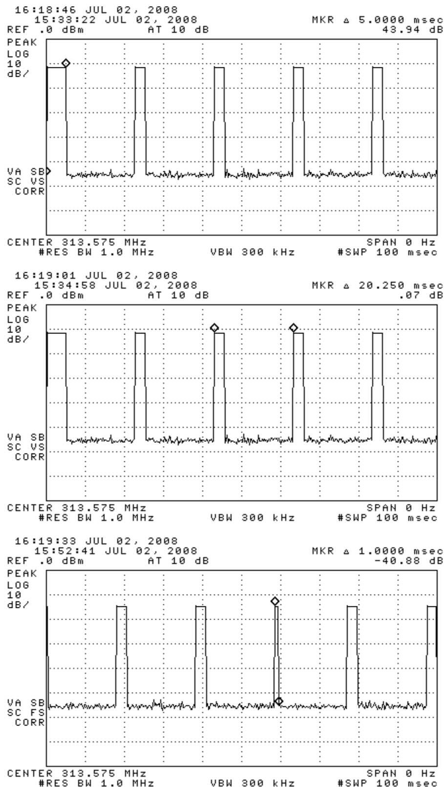
Figure 6.1(b). Transmissions modulation characteristics: leading PWM dataset (top) first bit, (center) period, (bottom) minimum PWM bit width.
