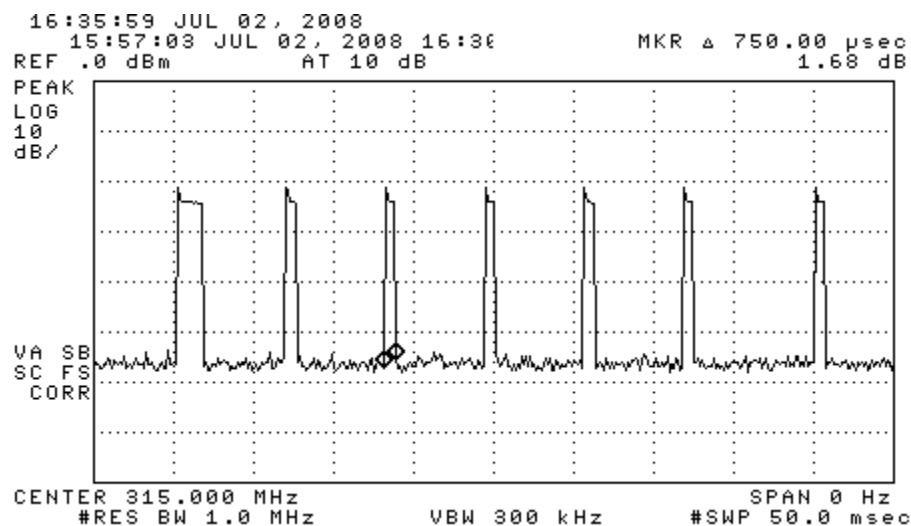
Figure 6.1(e). Transmissions modulation characteristics: Final dataset max PWM bit width.
