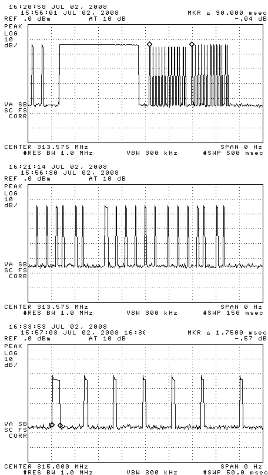
Figure 6.1(d). Transmissions modulation characteristics: Final PWM dataset (top) dataset, (center) one word of dataset, (bottom) leading pulse.
