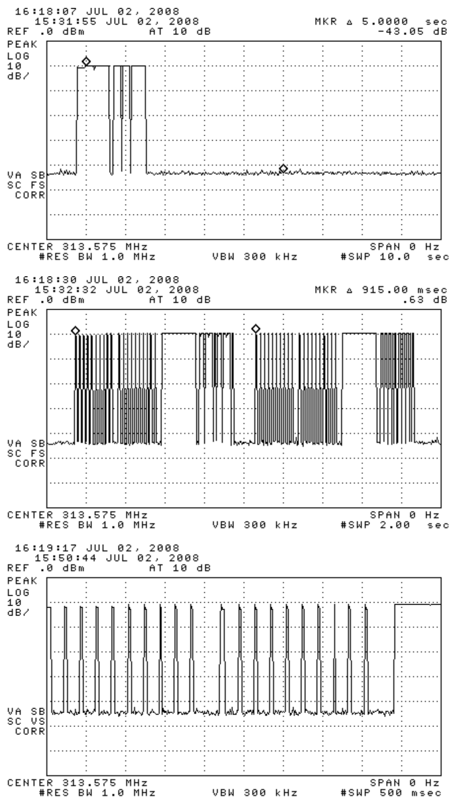
Figure 6.1(a). Transmissions modulation characteristics: (top) single button press, (center) two words with three data sets each, (bottom) leading dataset.
