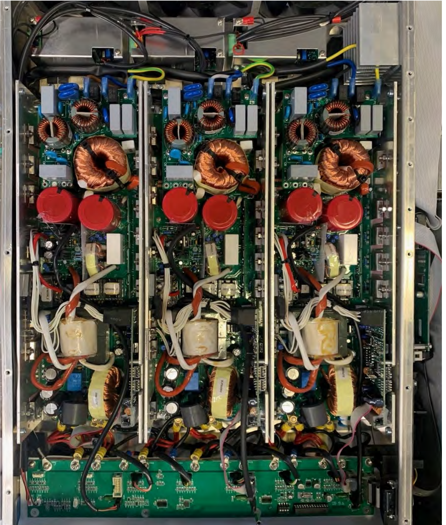
ETG5000 TOP VIEW
