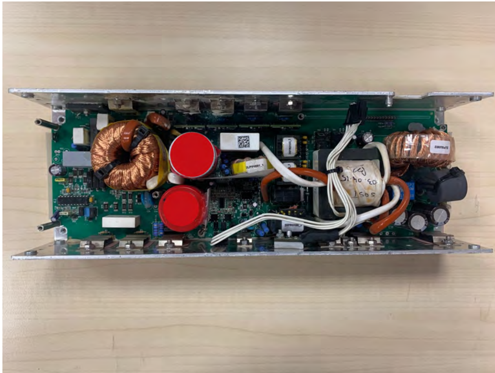
2K5W0A538-4 POWER SUPPLY BOARD SW. 2K5 PFC TOP
