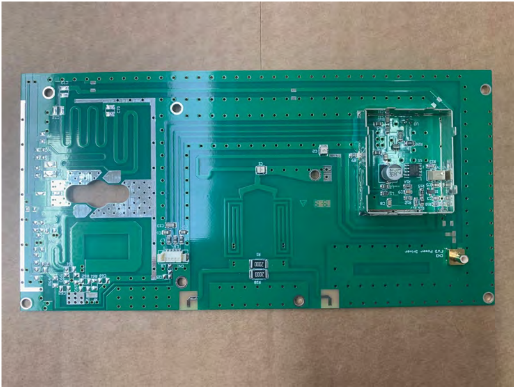
2U3KAB283-0 SPLITTER BOARD 2WAYS 1-1.5KW TOP
