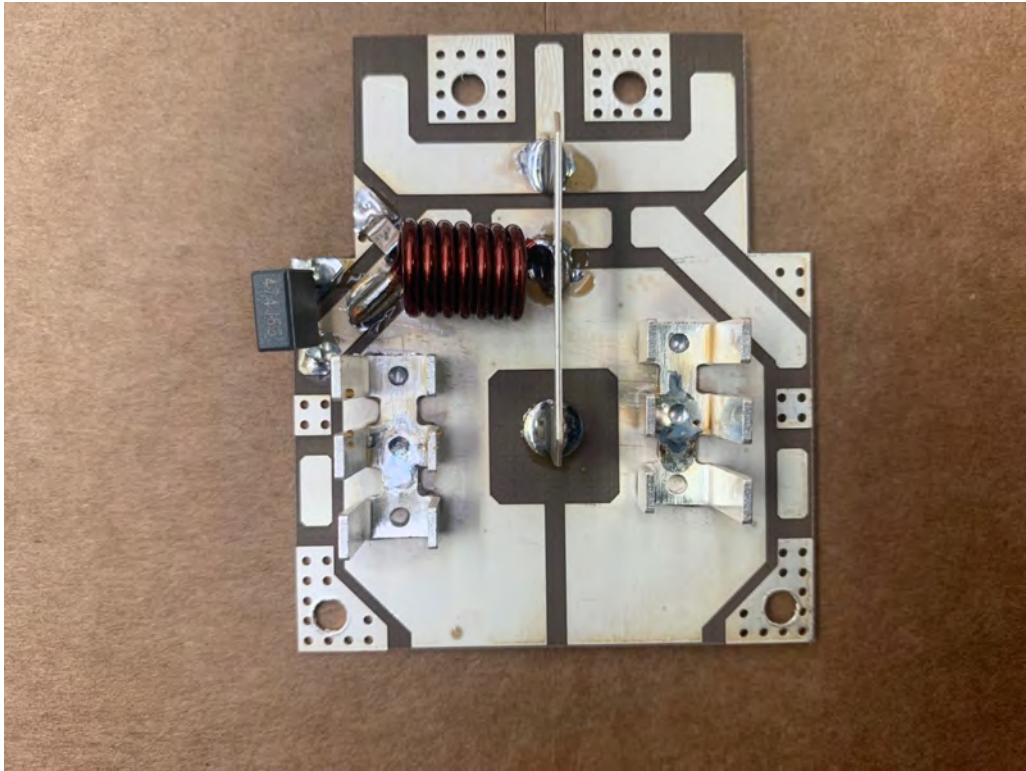
MAMP2A221-0 OUTPUT MODULE BOARD 800W TOP
