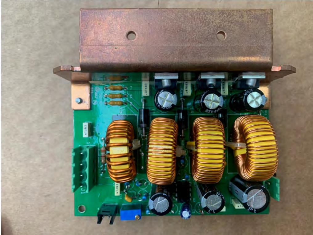
TG2UTA891-5 FAN POWER SUPPLY 3 SECTIONS TOP
