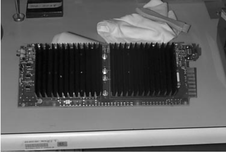
Power Amplifier Top View
