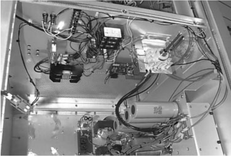
AC Distribution
