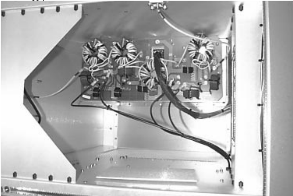
Combiner
