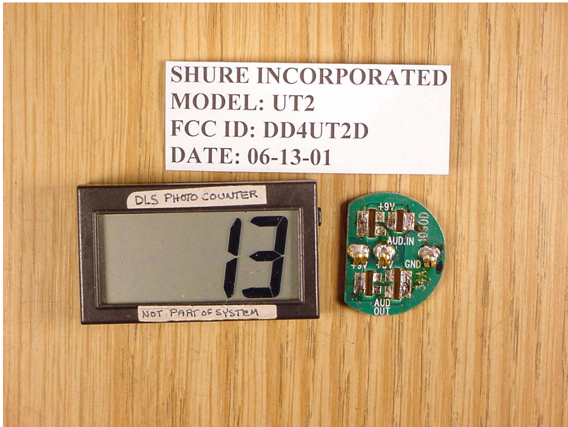
Interconnect Board Side 1
