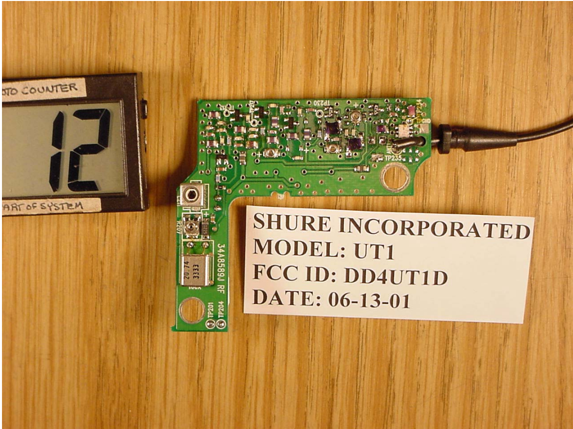
RF Board Component Side
