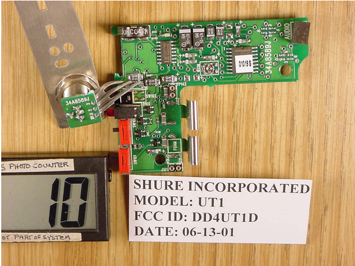
Audio Board Component Side
