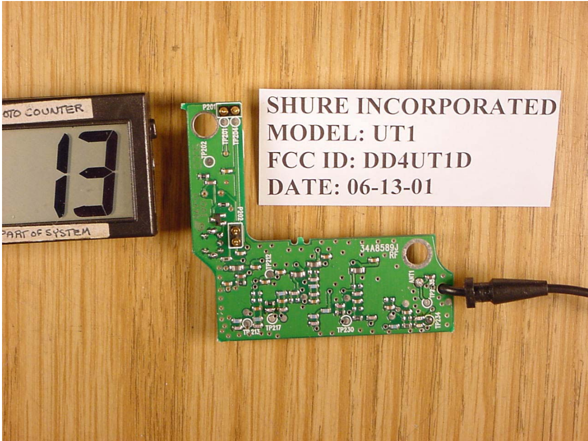
RF Board Solder Side
