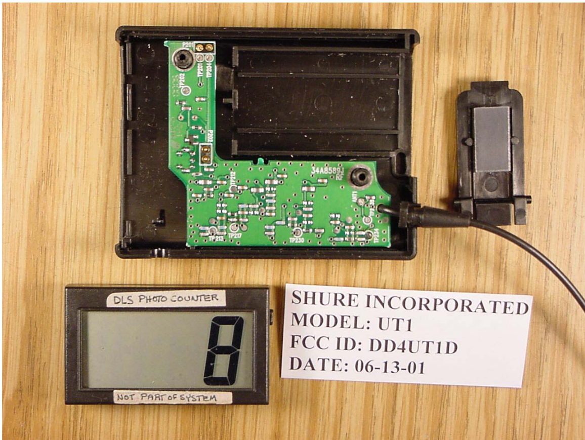
Audio Board removed
