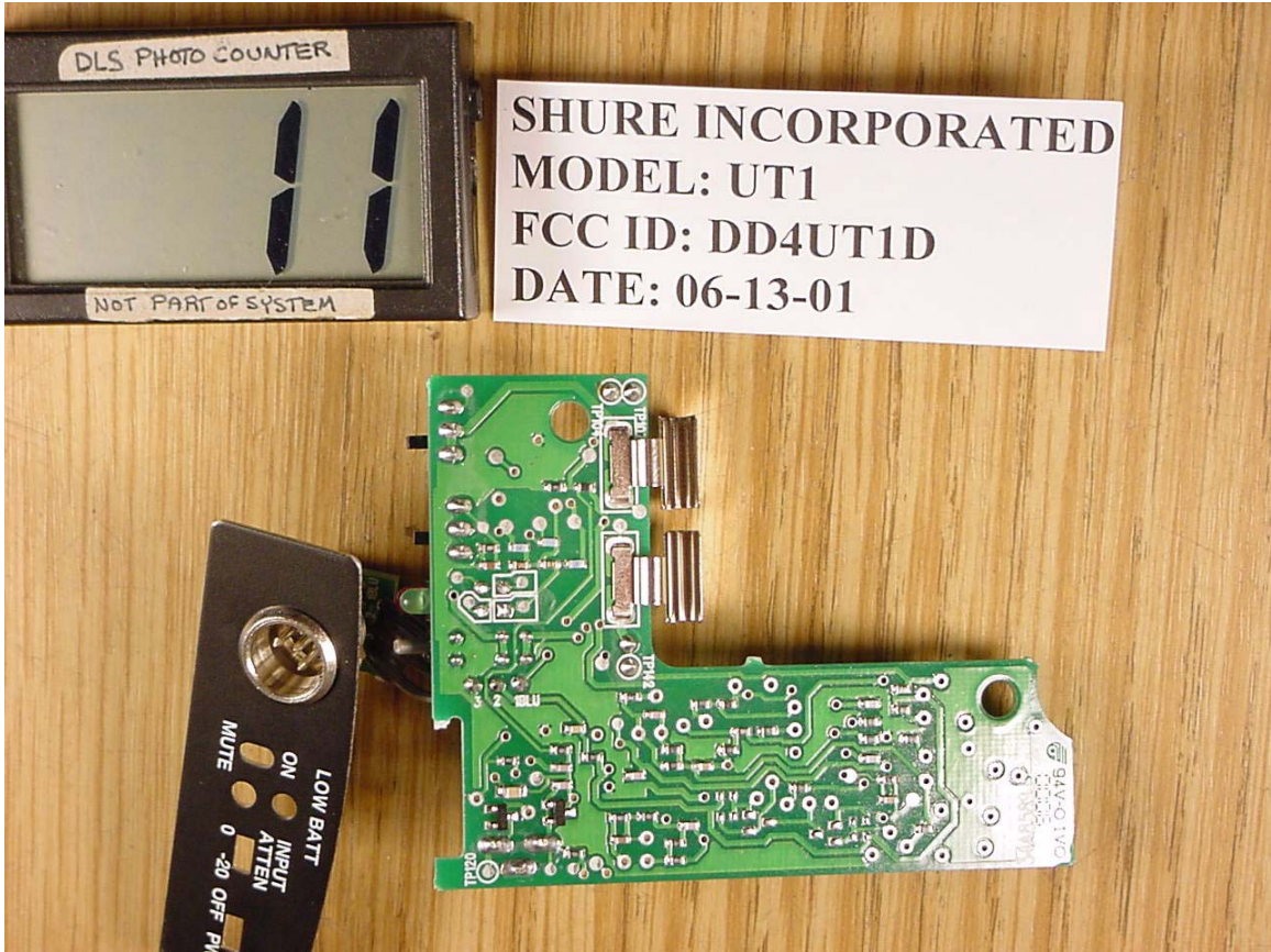
Audio Board Solder Side
