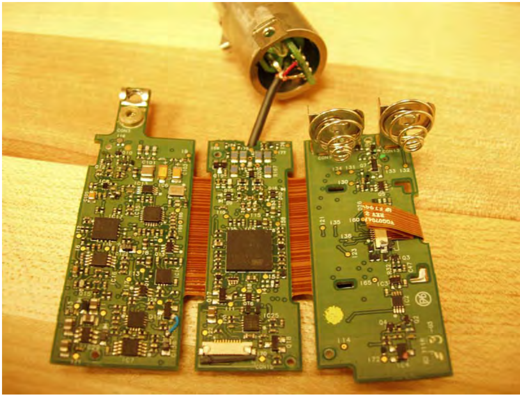
UR3 PCB Back
