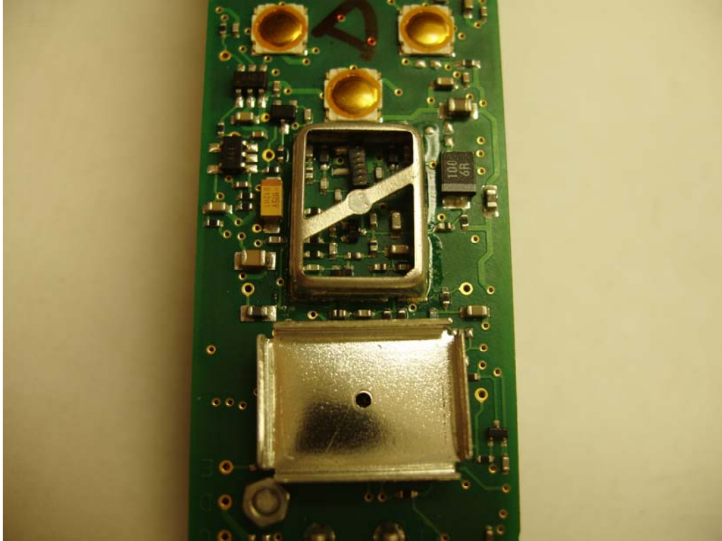
UR2A PCB RF Section
