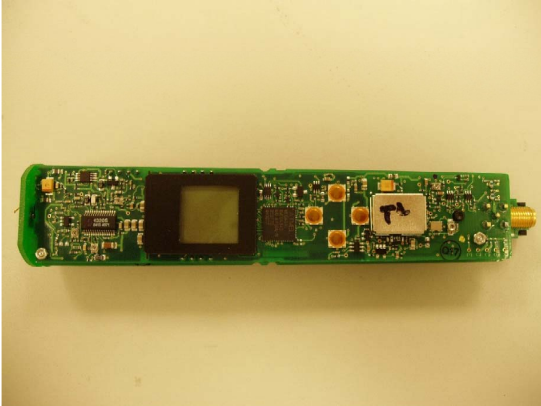
UR2A PCB Top Side
