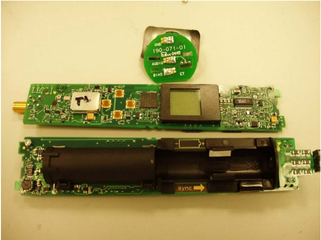
UR2A PCBs Outside
