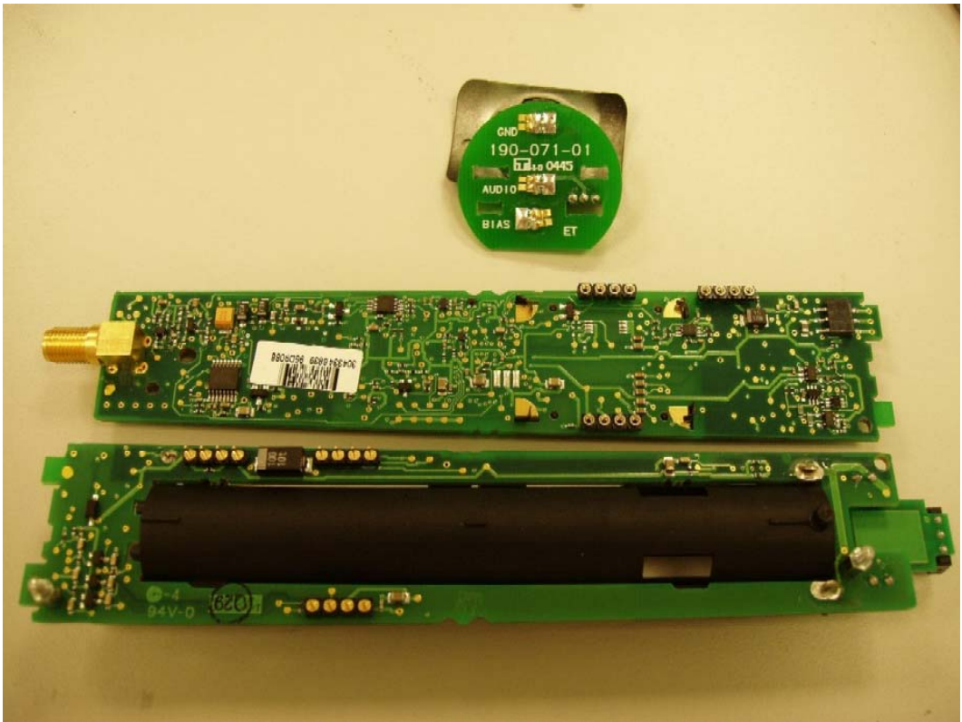
UR2A PCBs Inside
