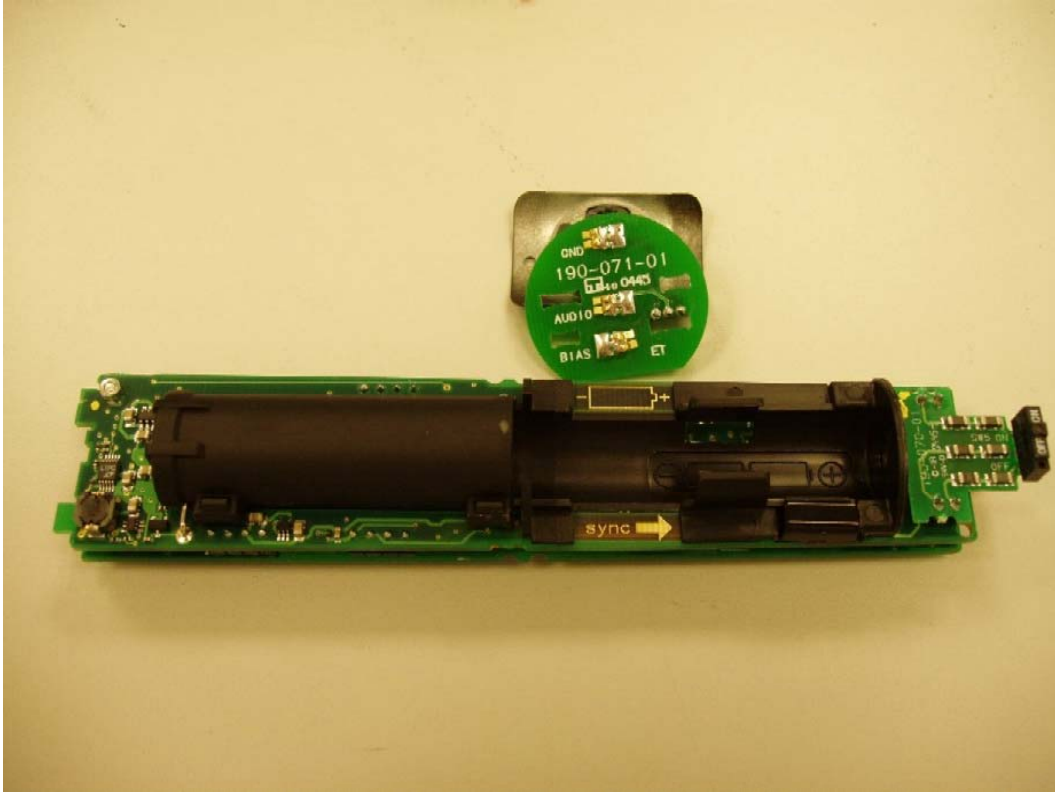
UR2A PCB Bottom Side
