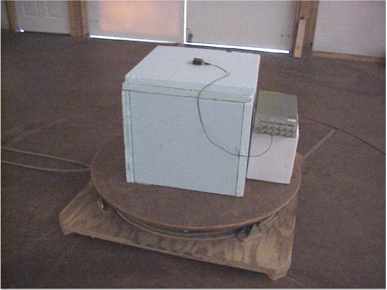
RADIATED SPURIOUS – Z ORIENTATION
