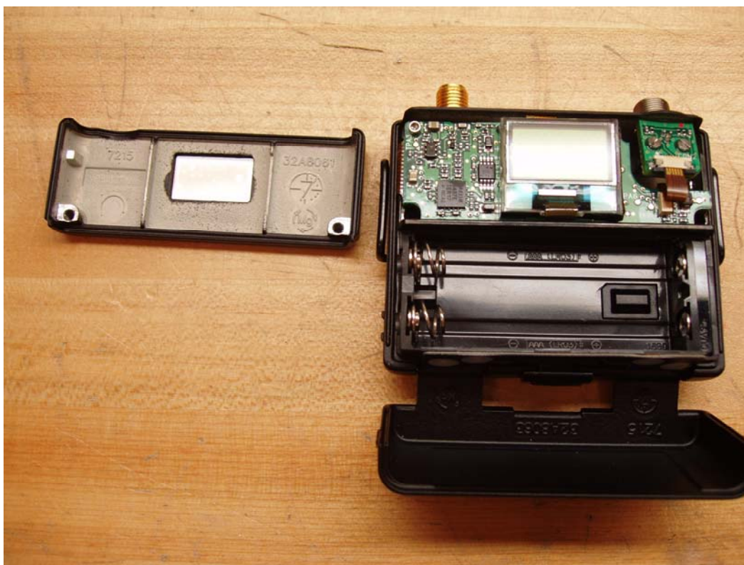
UR1M PCB Top in Case (All)
