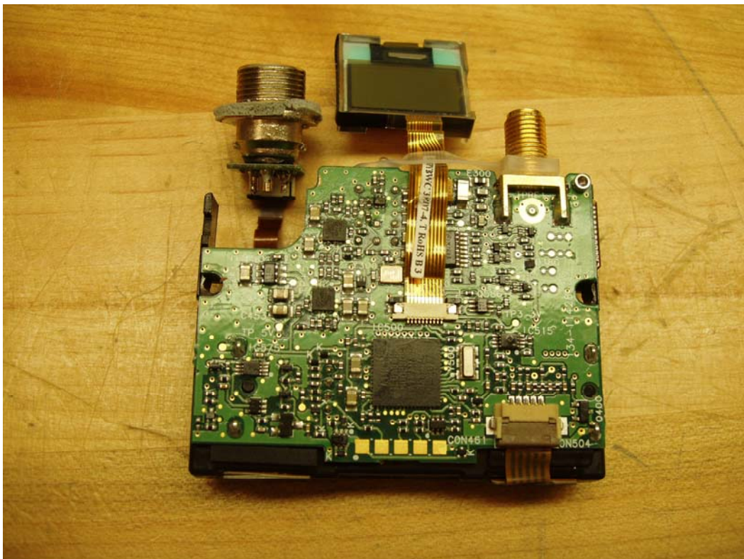
UR1M PCB Bottom (All)
