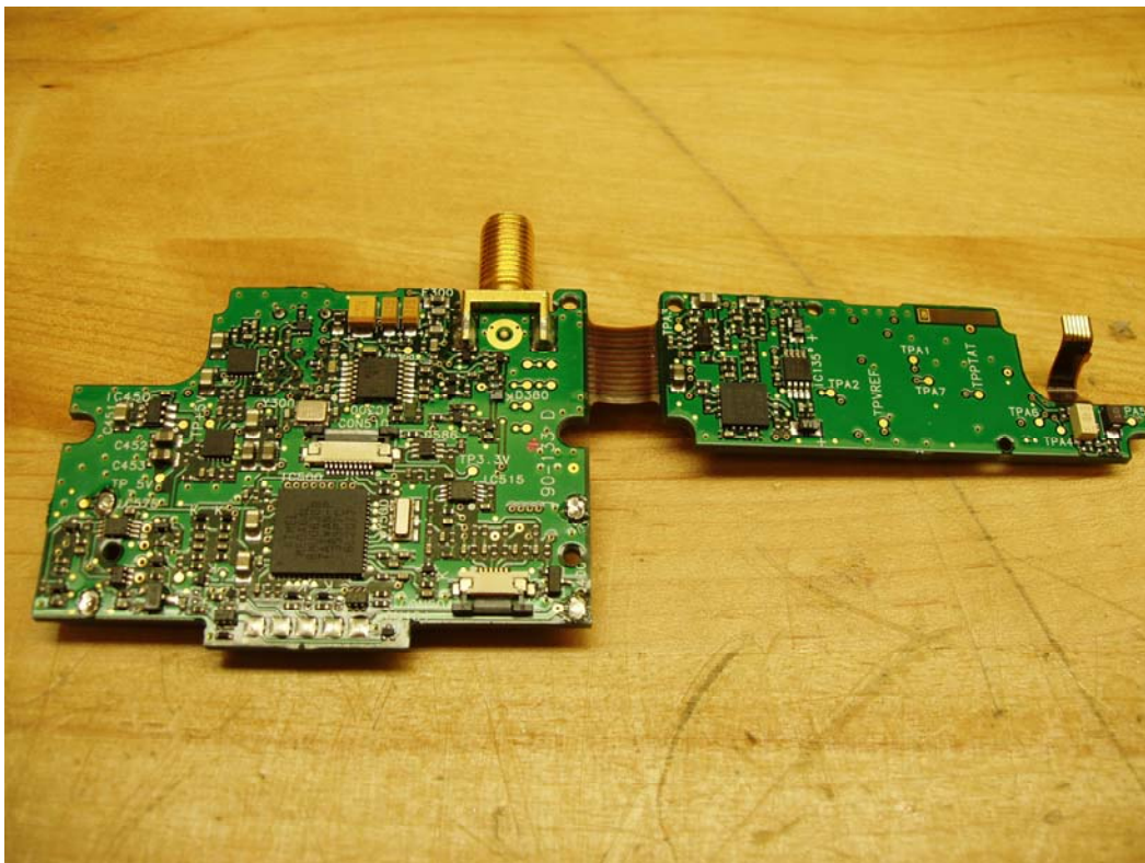
UR1M PCB Back – Audio & RF PCB open w/o ribbon cable (All)
