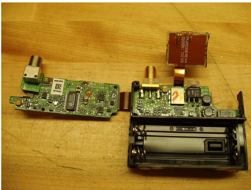
UR1M PCB – Audio & RF PCB open (All)
