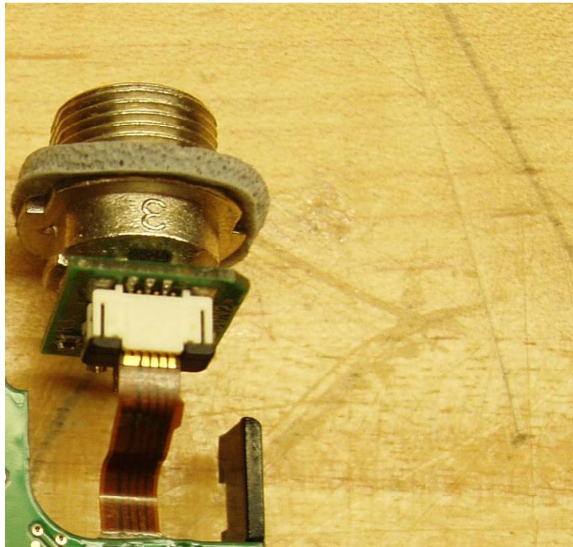
UR1M Microphone Connector PCB (TQG)
