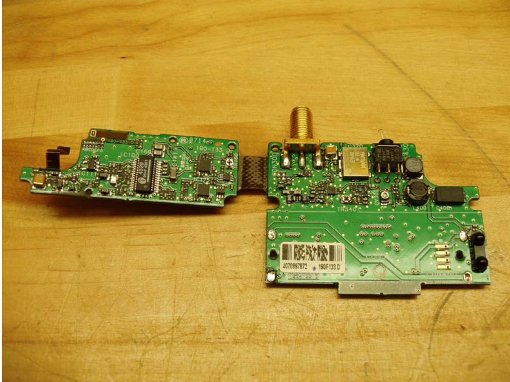
UR1M PCB – Audio & RF PCB open w/o Battery Holder (All)
