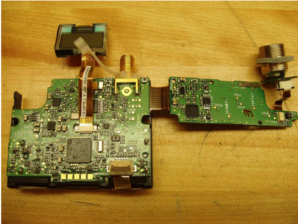
UR1M PCB Back – Audio & RF PCB open (All)
