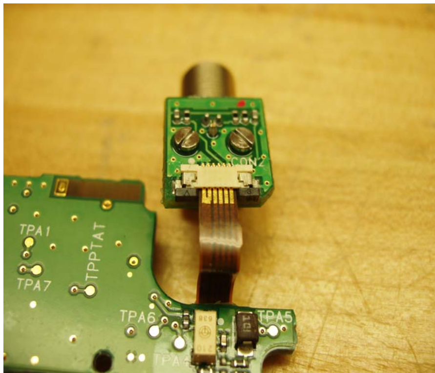
UR1M Microphone Connector PCB (LEMO3)
