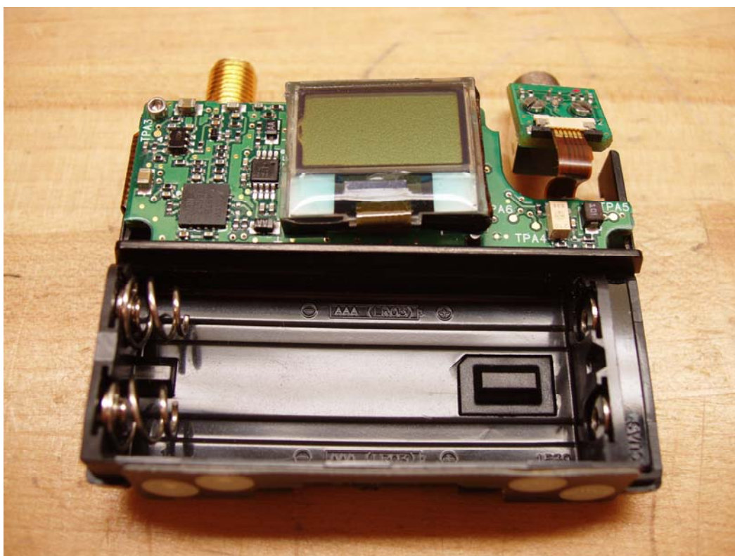
UR1M PCB Top (All)
