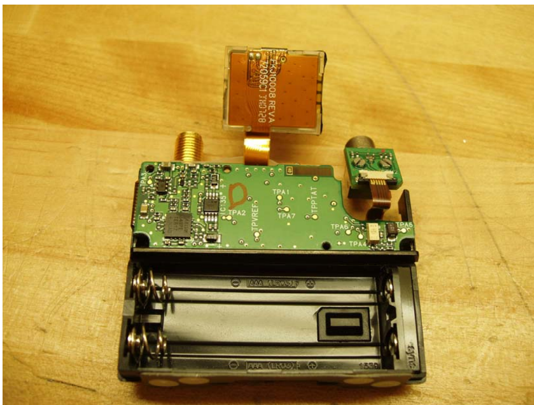
UR1M PCB Top – Under LCD (All)
