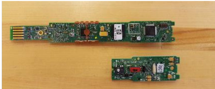
ULXD2 V50 Circuit Boards, Top
