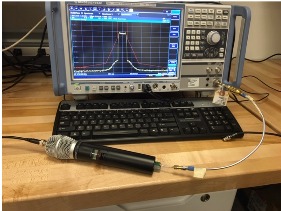
Test Setup for: Minimum Bandwidth, Spurious Emissions on Antenna Port and Test Setup for Power Spectral Density
