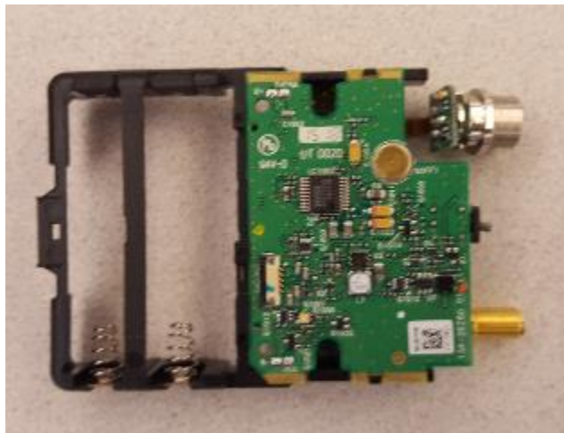
ULXD1 V50 Circuit Board Top
