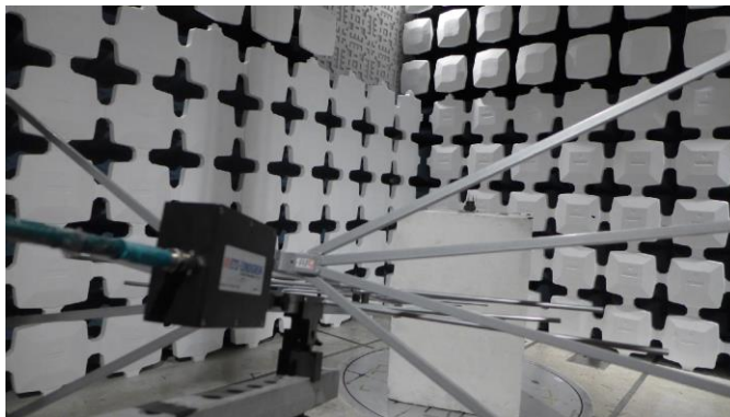
Figure 1: ULXD1 Transmitter Test Setup
