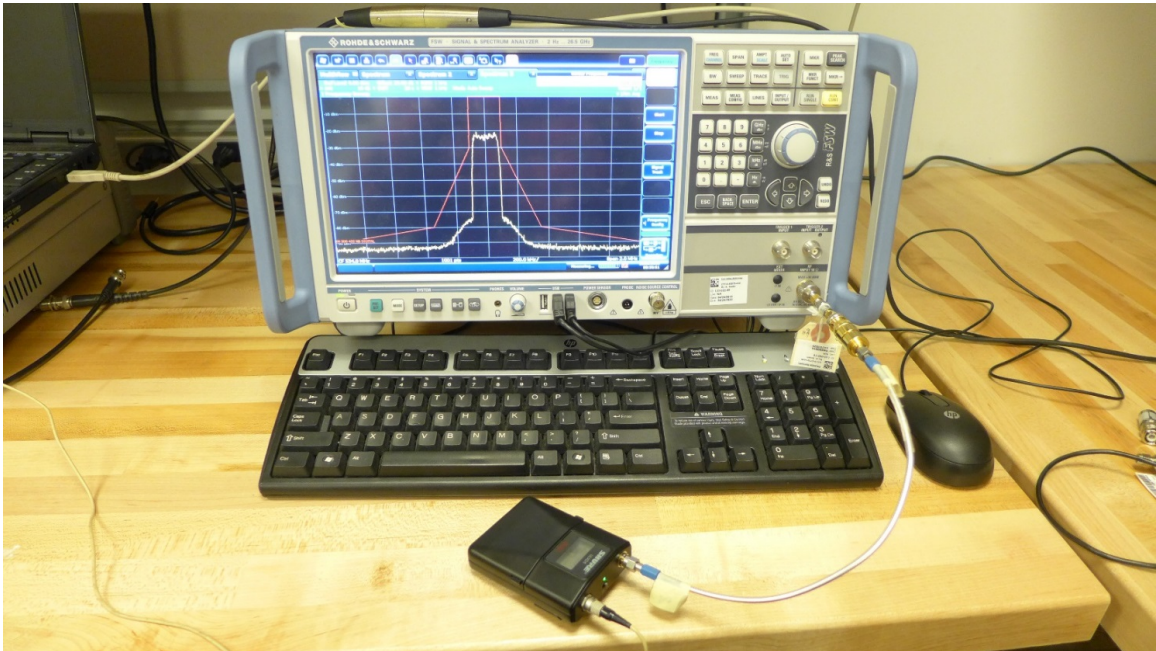
Test Setup for: Minimum Bandwidth, Spurious Emissions on Antenna Port and Test Setup for Power Spectral Density
