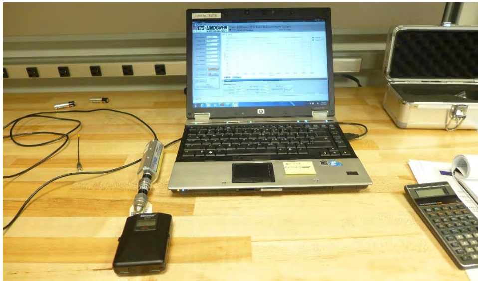
Figure C 1: Test setup for Maximum Power Output
