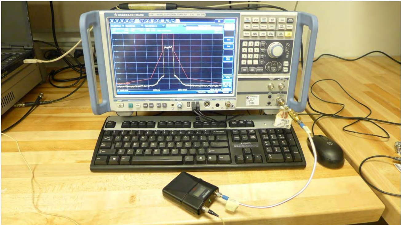
Figure A-1 - Test Setup for Necessary Bandwidth
