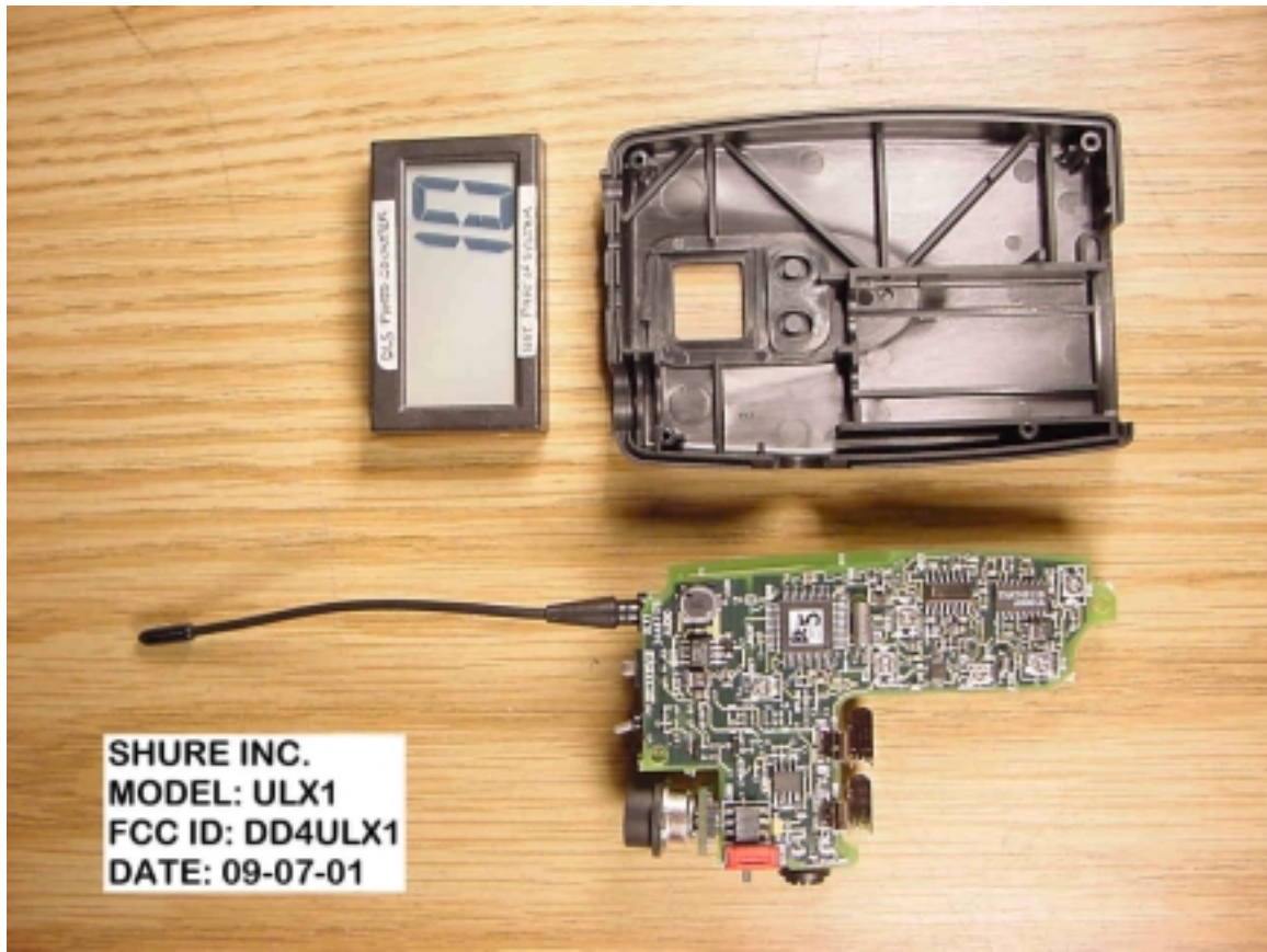
FRONT COVER REMOVED
