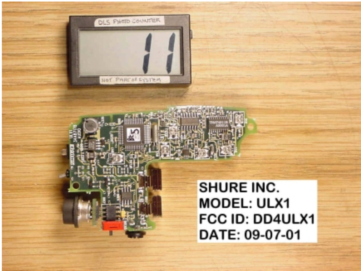
AUDIO BOARD SIDE #1
