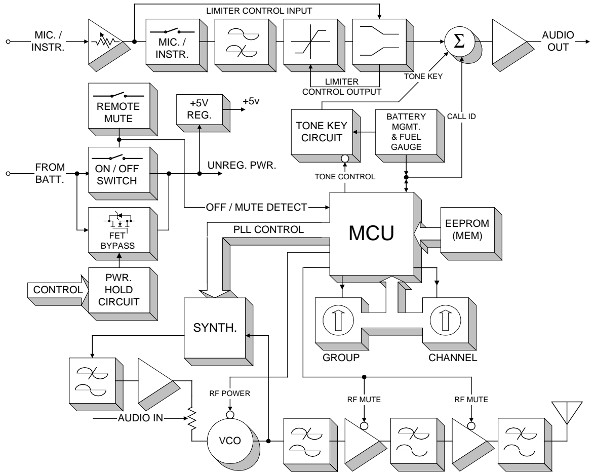
Figure 1 Block Diagram of the UC1B Body Pack Transmitter
