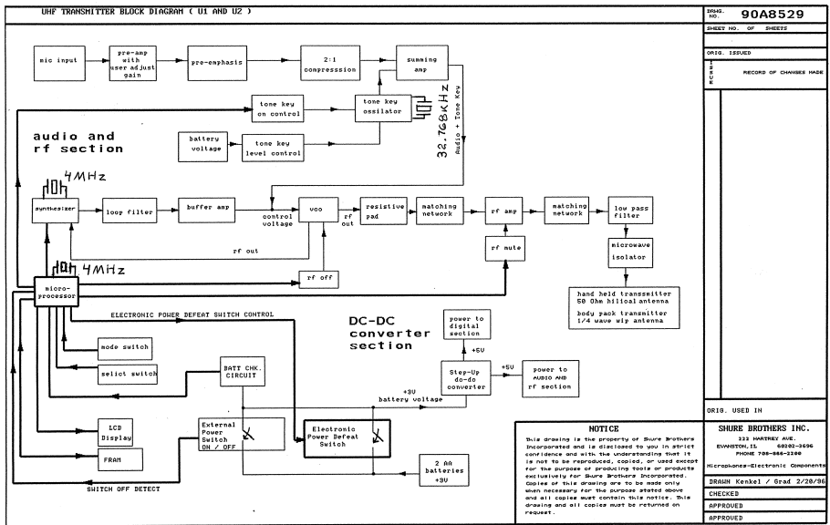
U1B Block Diagram
