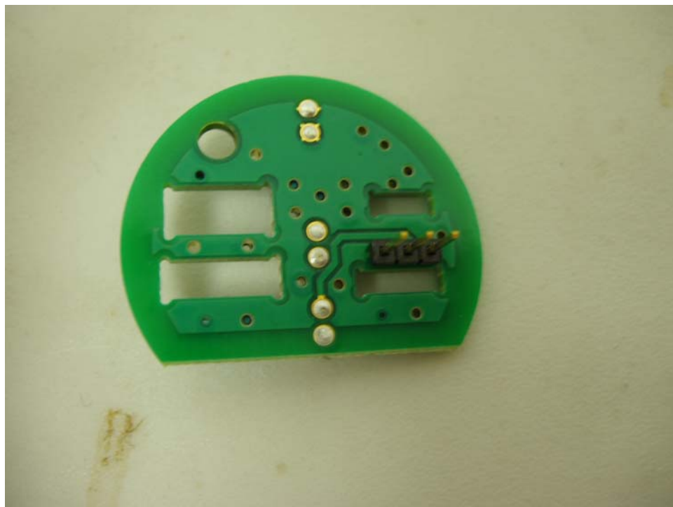
FP2 Audio Input - Bottom
