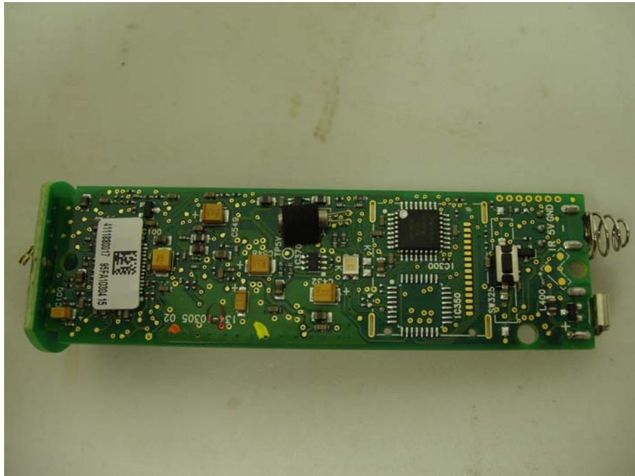
FP2 PCB Back
