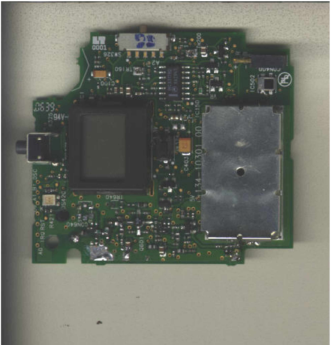
PC Board Side 1 with shield
