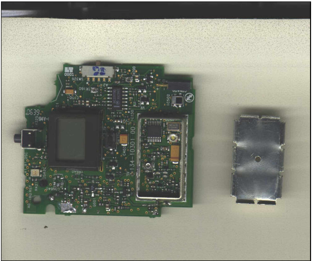
PC Board Side 1 with Shield Removed
