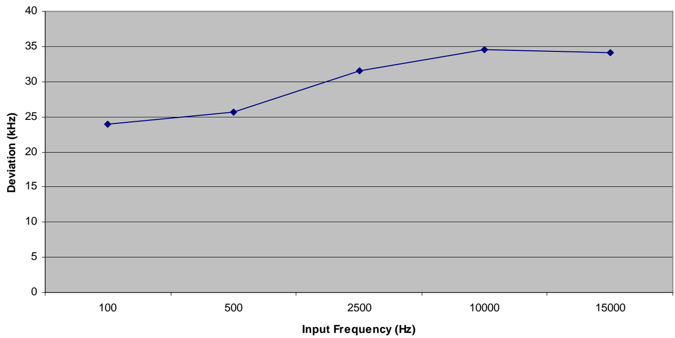
SLX1 G4 Deviation vs. Input Frequency (-40 dBu Input with 0dB Gain Setting)
