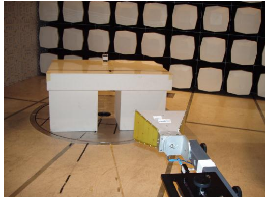
Figure D-2. QLXD1 in Semi-Anechoic Chamber
