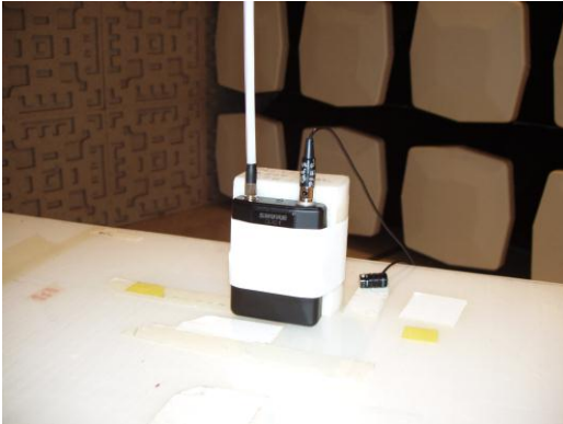
Figure D-1. QLXD1 in Semi-Anechoic Chamber
