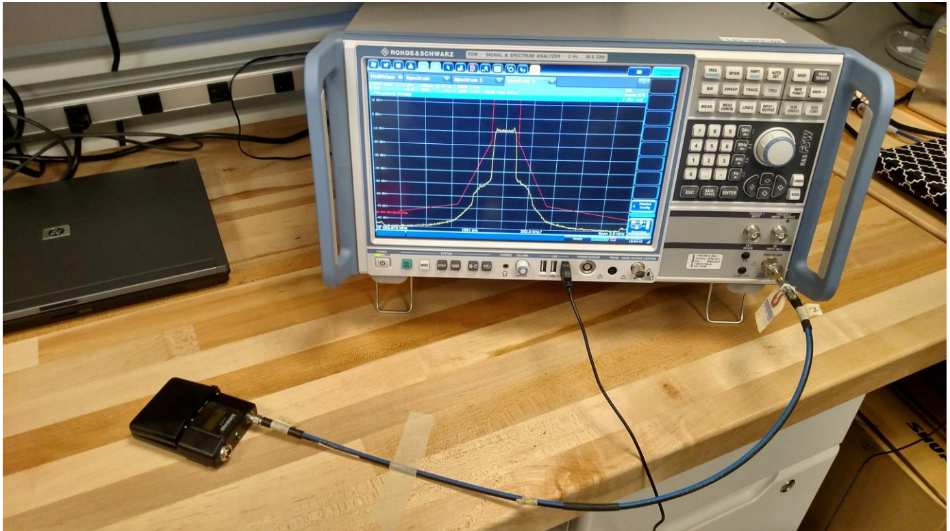
Figure B-1 - Test Setup for Necessary Bandwidth
