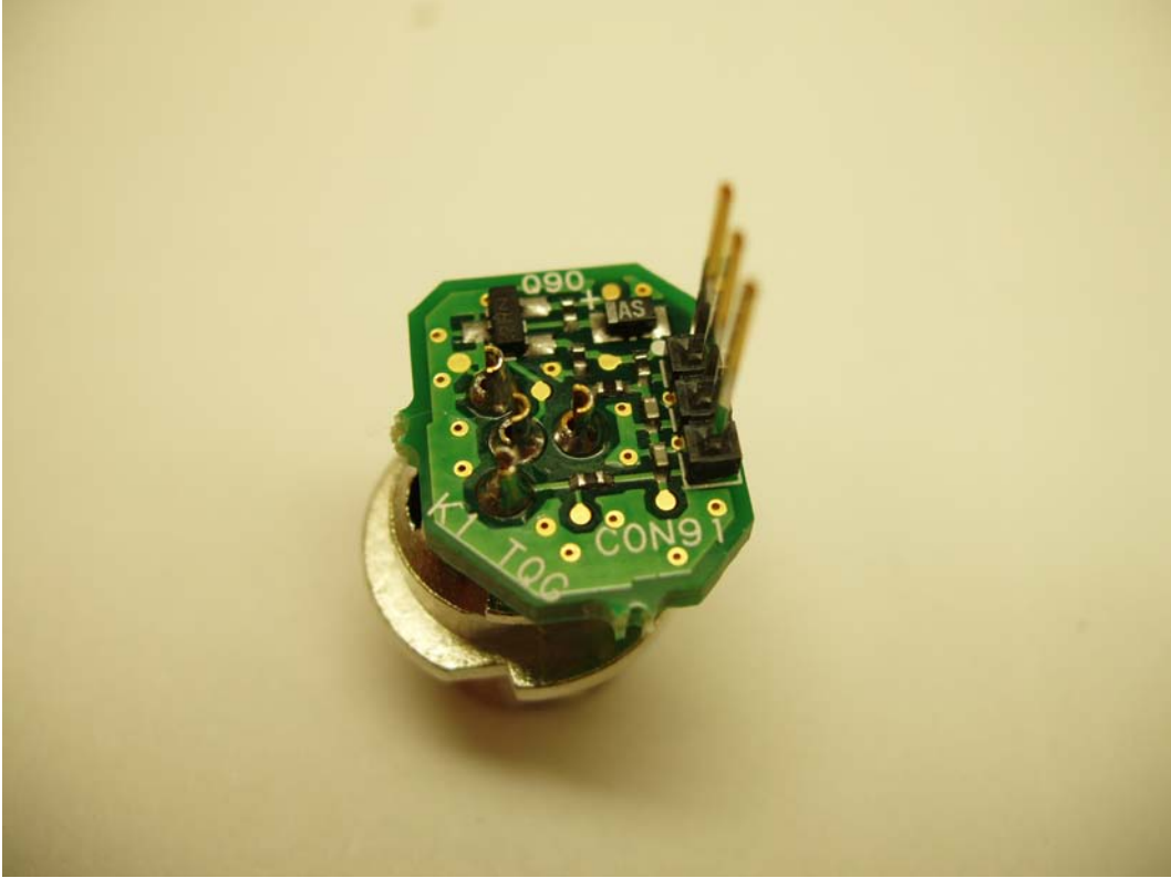
PGXD1 Microphone Connector PCB
