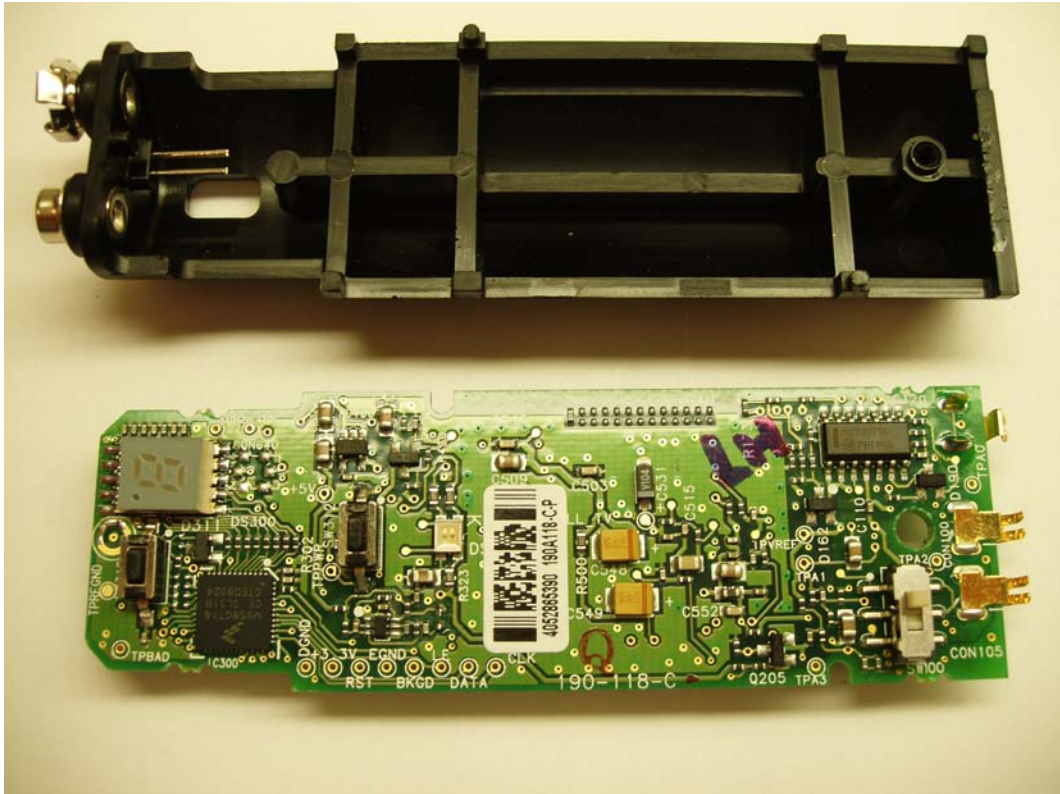
PG2 PCB Topside
