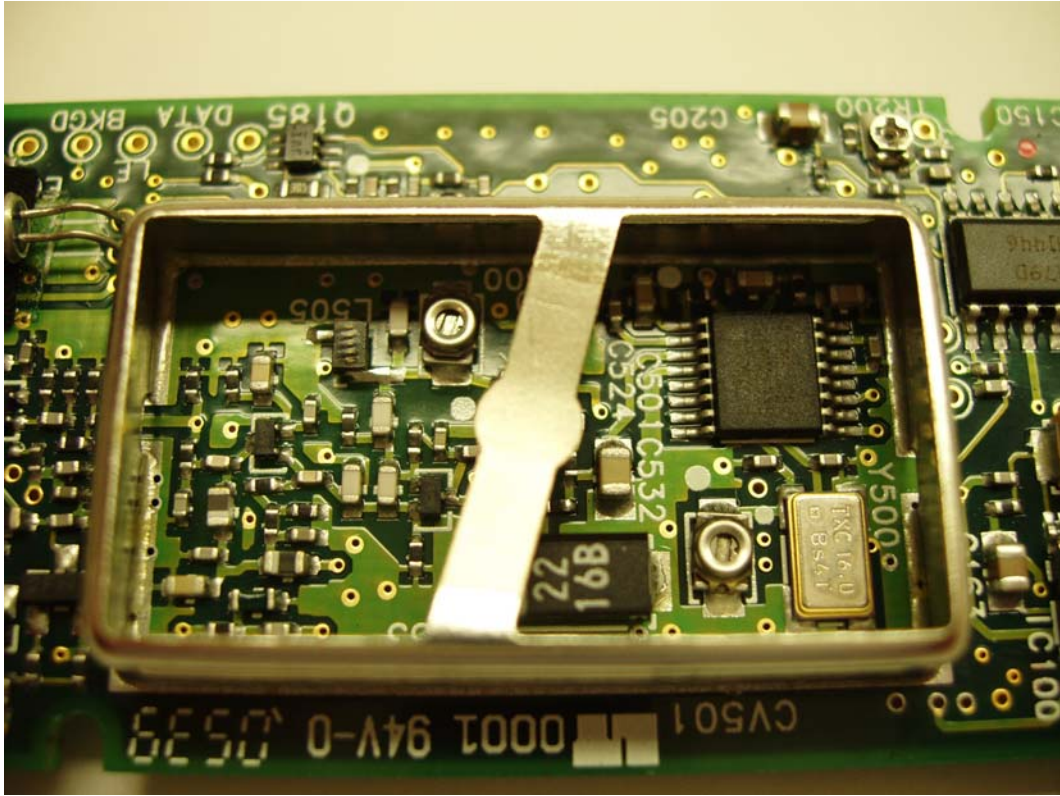
PG2 PCB RF Section
