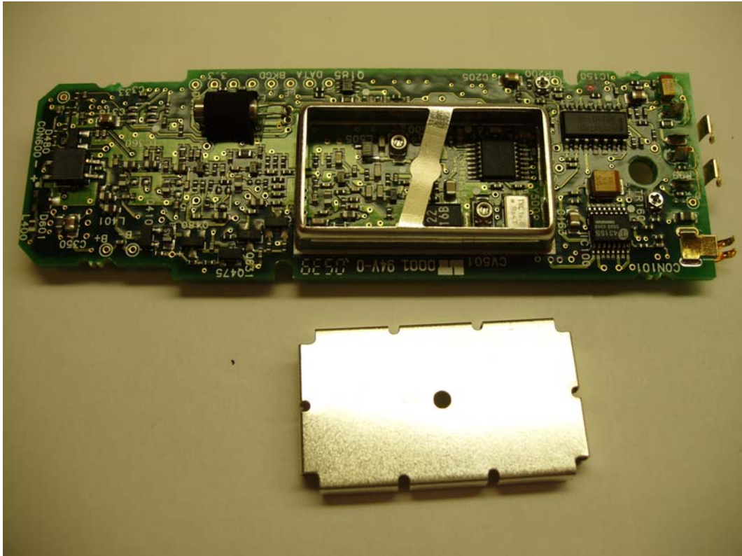
PG2 PCB Bottom Side with Shield Removed
