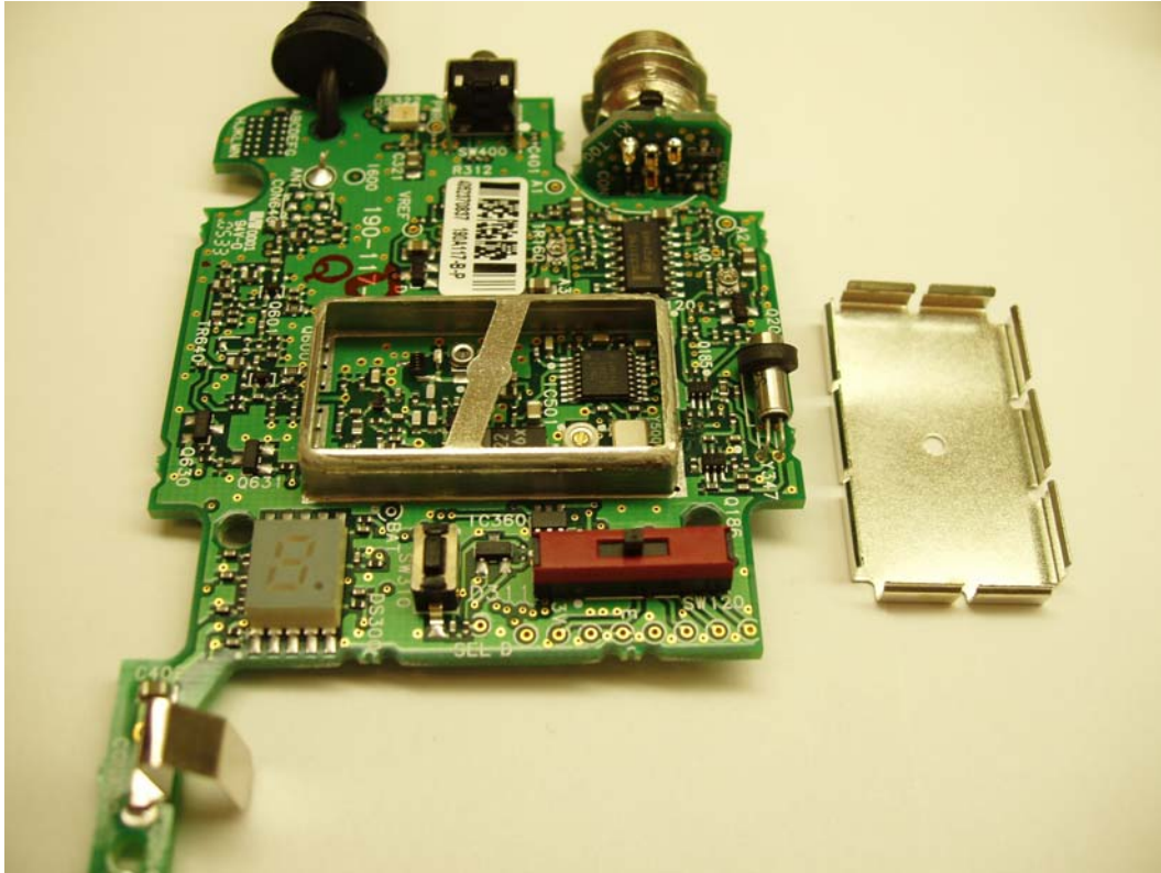
PG1 PCB Top without Shield
