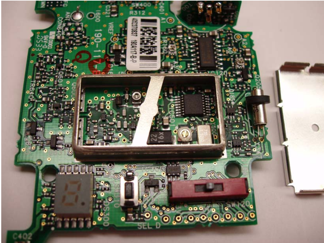
PG1 PCB RF Section
