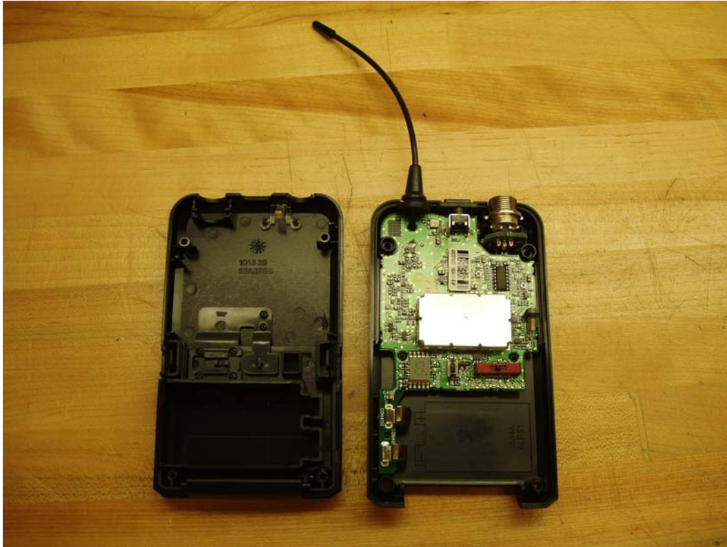
PG1 PCB Top in Case
