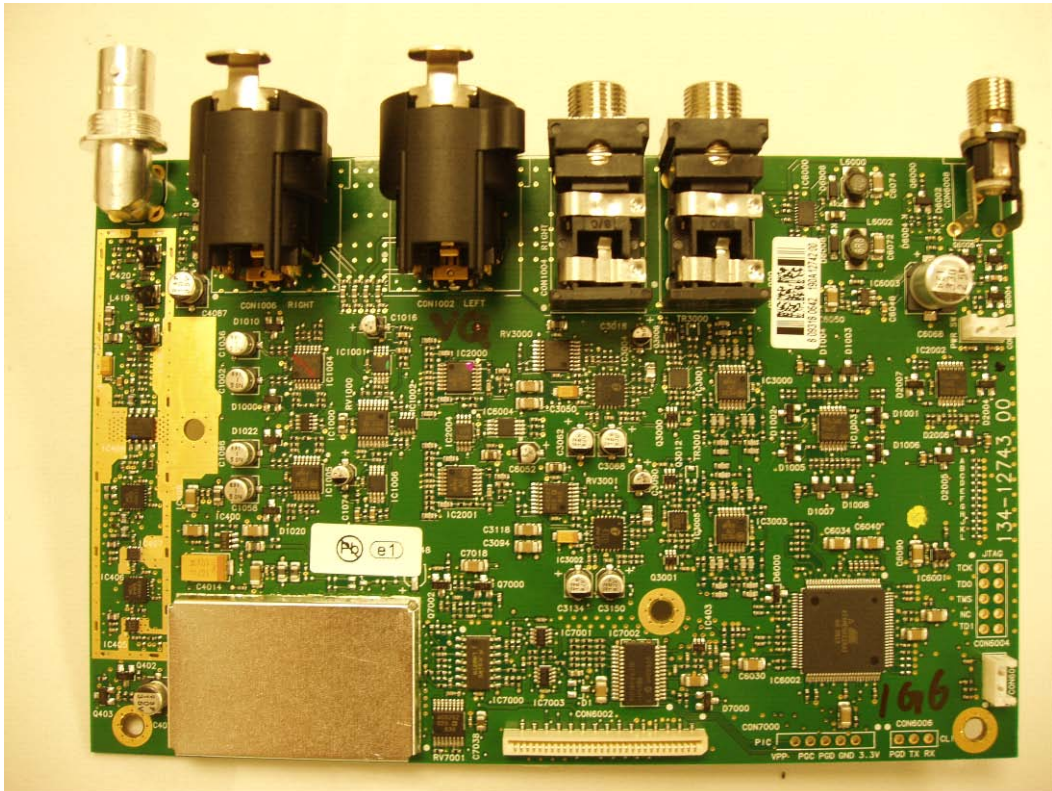
P9T PCB Top
