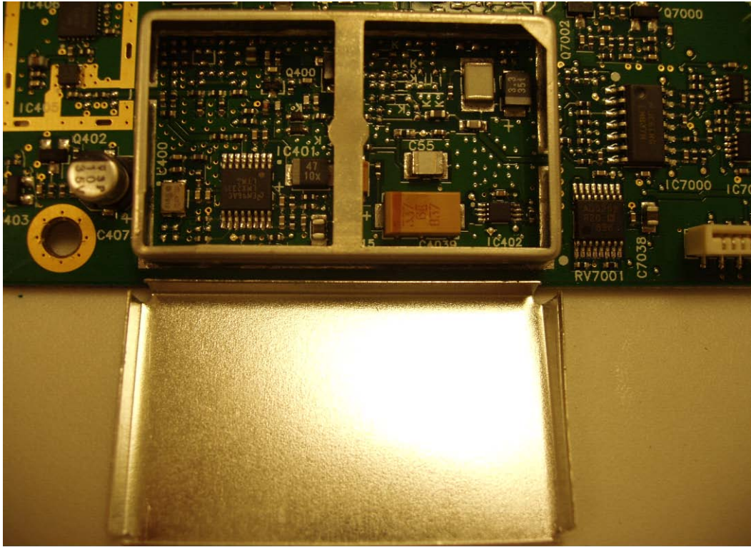
P9T PCB Top (Shield removed)
