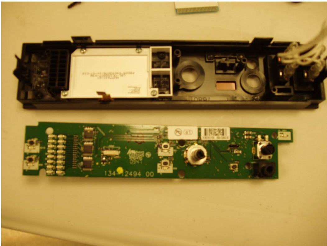
P9T Front Panel PCB
