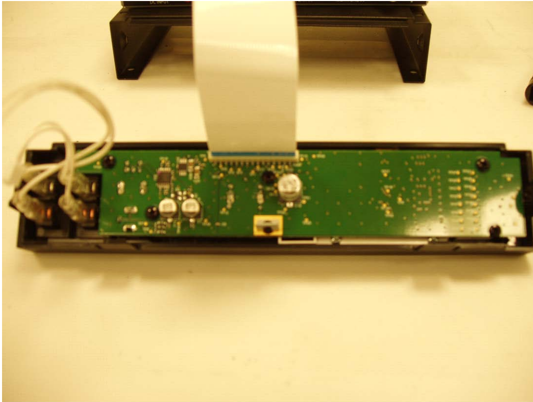
P9T Front Panel PCB (Back)
