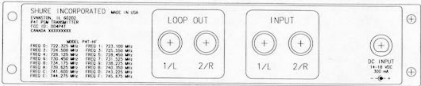
95HF8867 REAR PANEL ASSEMBLY
