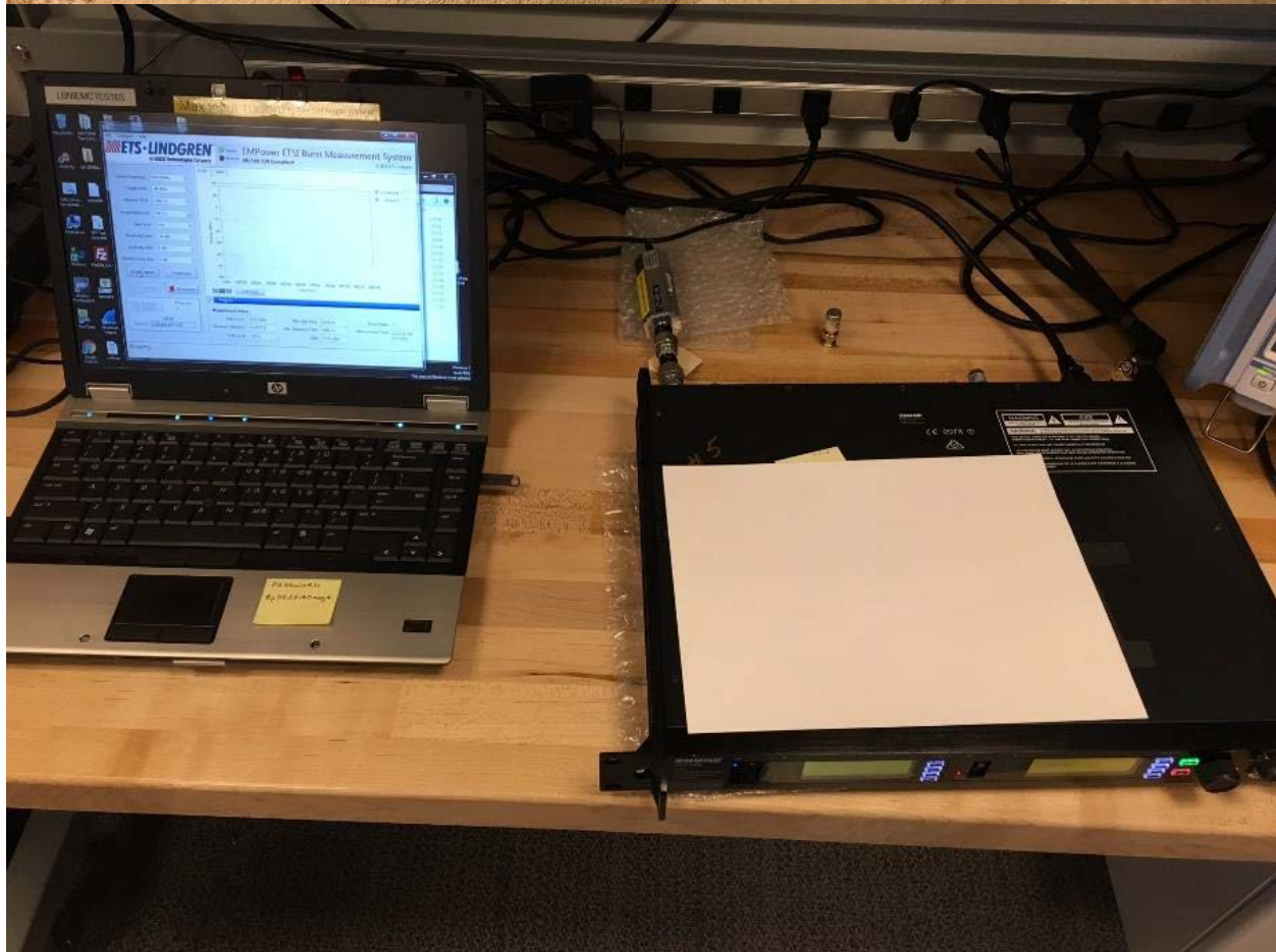
RF OUTPUT POWER TEST SETUP
