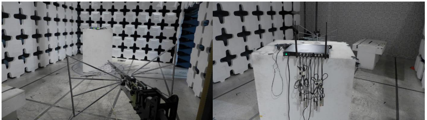
Figure 1: P10T Transmitter Test Setup
