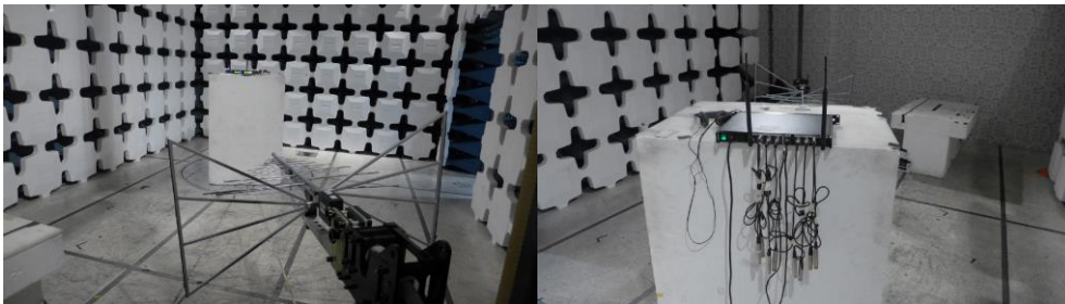
Figure 1: P10T Transmitter Test Setup
