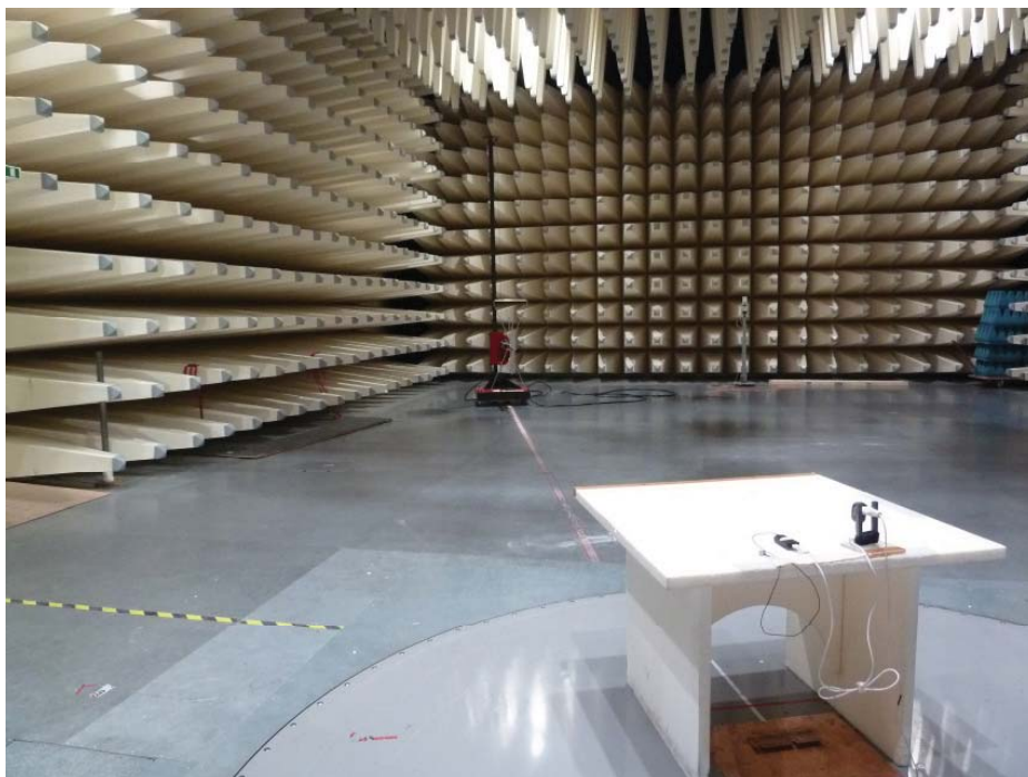
Photo 2: Radiated Emission
