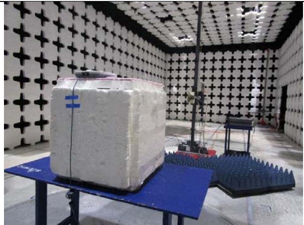
Radiated Emissions Above 1 GHz – Rear View
