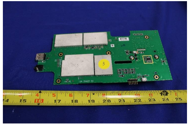
Modem Board-1 Bottom View
