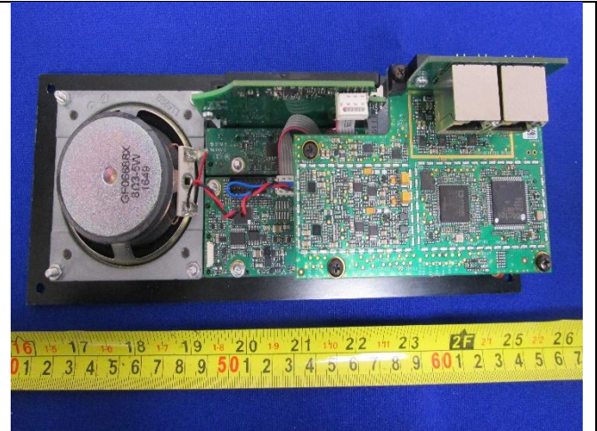
EUT Open Case View 2
