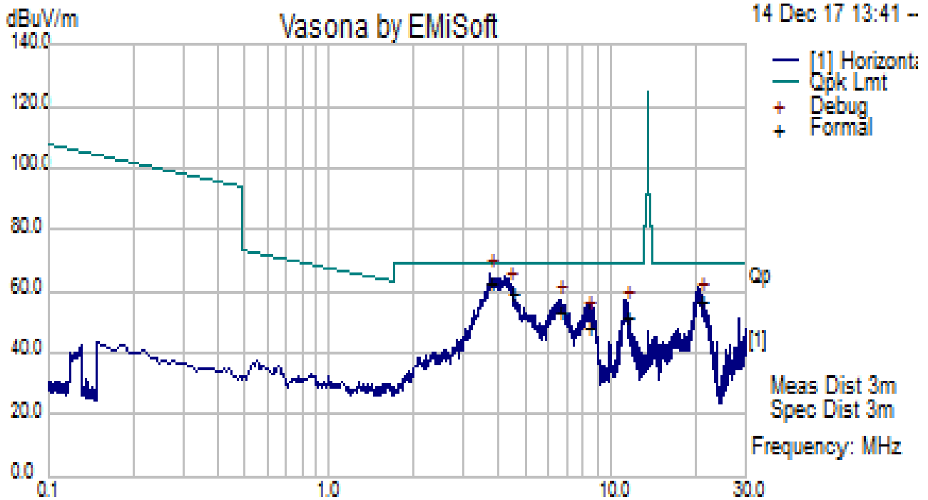
Quasi Max Measurement
