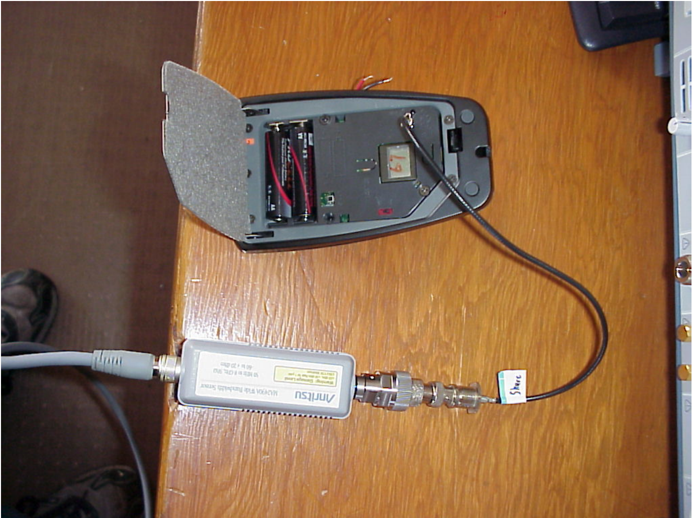
CONDUCTED OUTPUT POWER FCC
