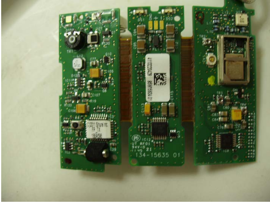
FP3 PCB Top
