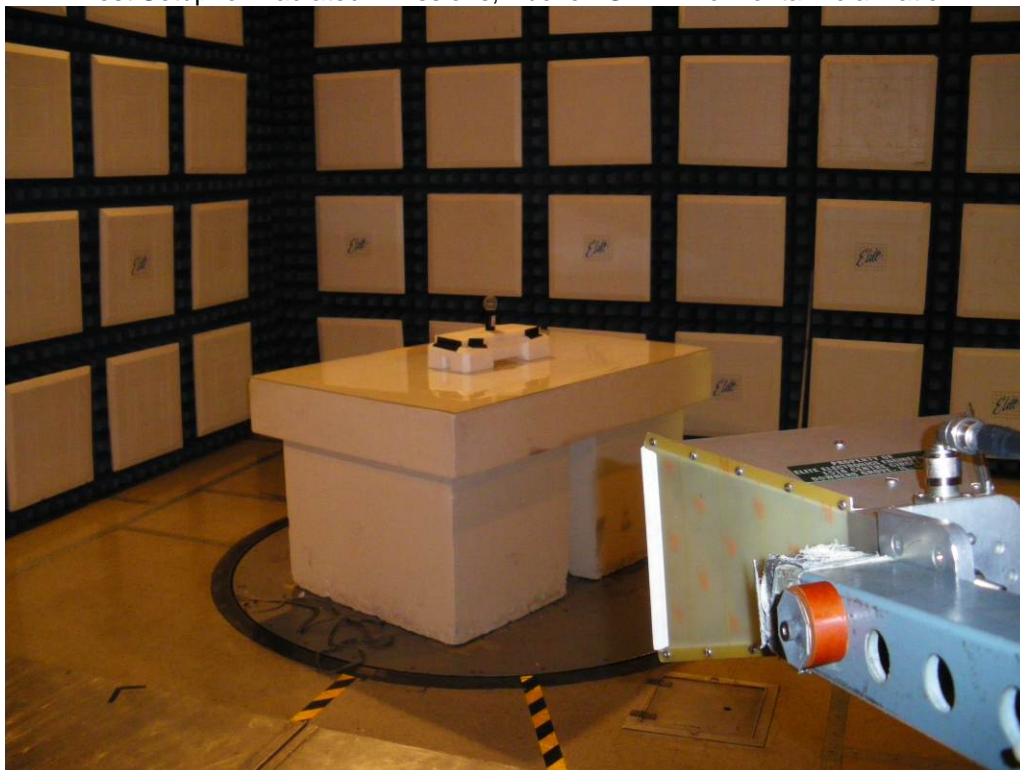
Test Setup for Radiated Emissions, Above 1GHz – Vertical Polarization Figure 4
